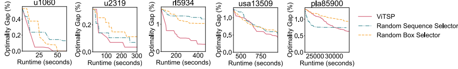
Figure 3: Ablation studies of different selection policies on selected instances.
