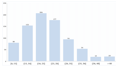
Fig. 8: Instruction length distribution
