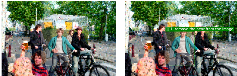
Fig. 14: The left image shows the editing result, and the right image visualizes the editing region on top of the result. We mask out the background patches’ attention to the global prompt token, and find that the image patches unable to attend to any text tokens exhibit severe distortion.
