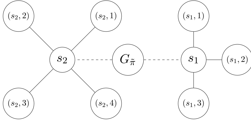
FIGURE 3. Modifying the graph G_{\tilde{\pi}} to construct \tilde{G}_{\tilde{\pi}} . Here, we pick two vertices s_1, s_2 \in V_{\tilde{\pi}} , with \tilde{n}_{s_1} = 3, \tilde{n}_{s_2} = 4 .
