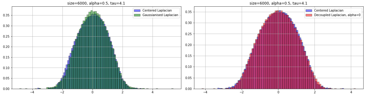
FIGURE 2. Comparing the spectrum of the centred Laplacian with the Gaussianised and the decoupled case.
