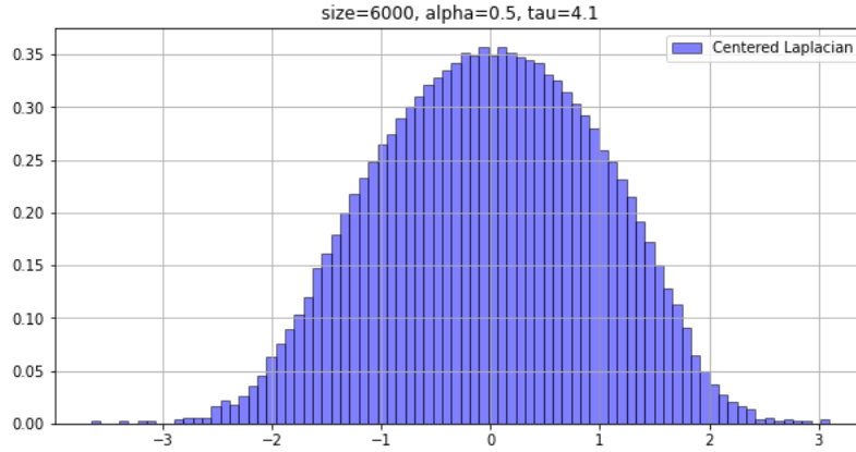
FIGURE 1. Spectrum of the centred Laplacian matrix .
