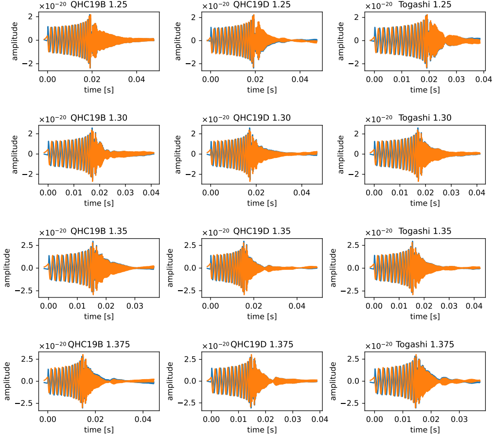
Figure 7: 12 BNS waveform models by Huang et al.[31]. Blue and orange lines are h_+ and h_\times modes respectively.
