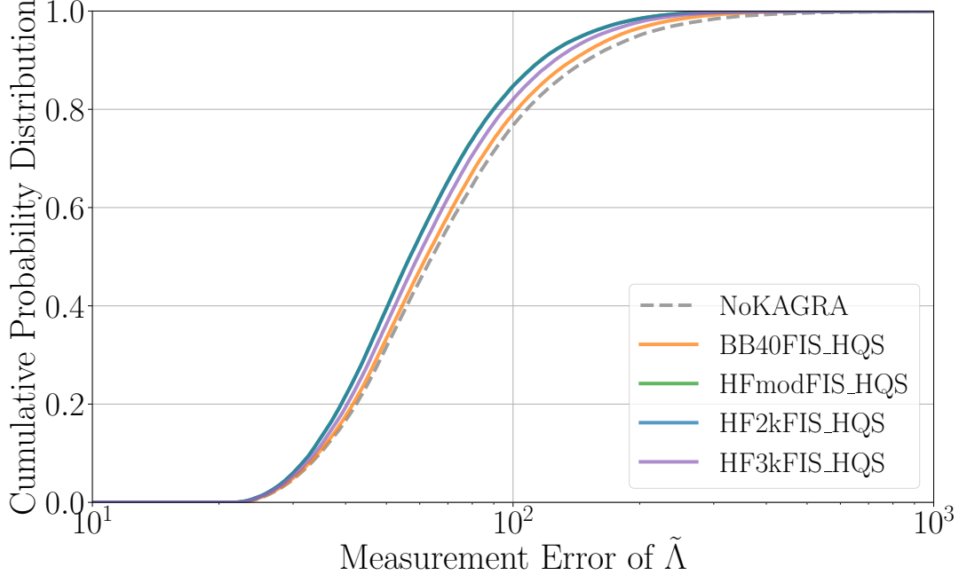
Figure 3: Cumulative distributions of measurement errors in \tilde{\Lambda} for 1.4M_{\odot}-1.4M_{\odot} BNSs at a luminosity distance of 200 Mpc, observed with the LIGO-KAGRA detector network under various KAGRA configurations. The results for HFmodFIS_HQS and HF2kFIS_HQS are nearly identical, and their curves overlap.
