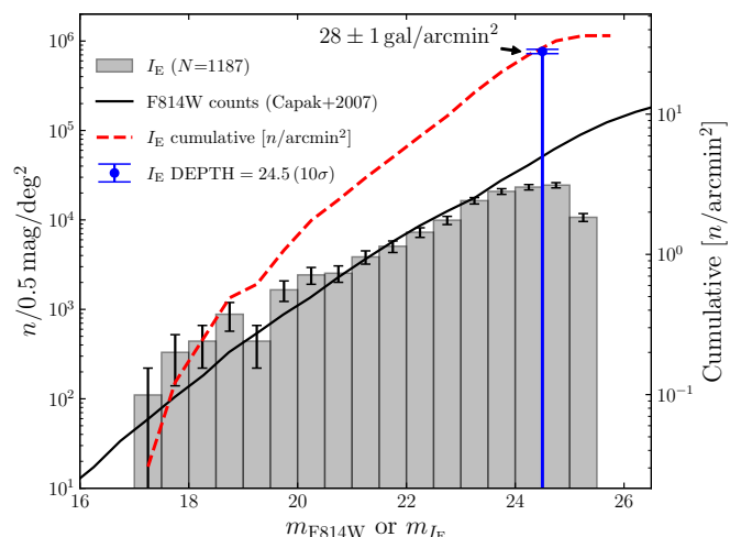
Fig. 5. Galaxy number counts from Euclid observations. The galaxy differential number counts derived from the simulated Euclid observations in the I_{\text{E}} band of the six HFF parallel fields are shown by the grey histogram with error bars. For comparison, those measured from HST observations ( Capak et al. 2007 ) are indicated by the black solid line. The vertical blue line marks the limiting magnitude in the I_{\text{E}} band (24.5 at 10\sigma ). The cumulative number of galaxies per arcmin 2 is shown by the red dashed line. We estimate the number counts from a total area of \sim 32.67 \text{ arcmin}^2 . We quote the number of galaxies per arcmin 2 at the limiting magnitude at the top of the blue vertical line.
