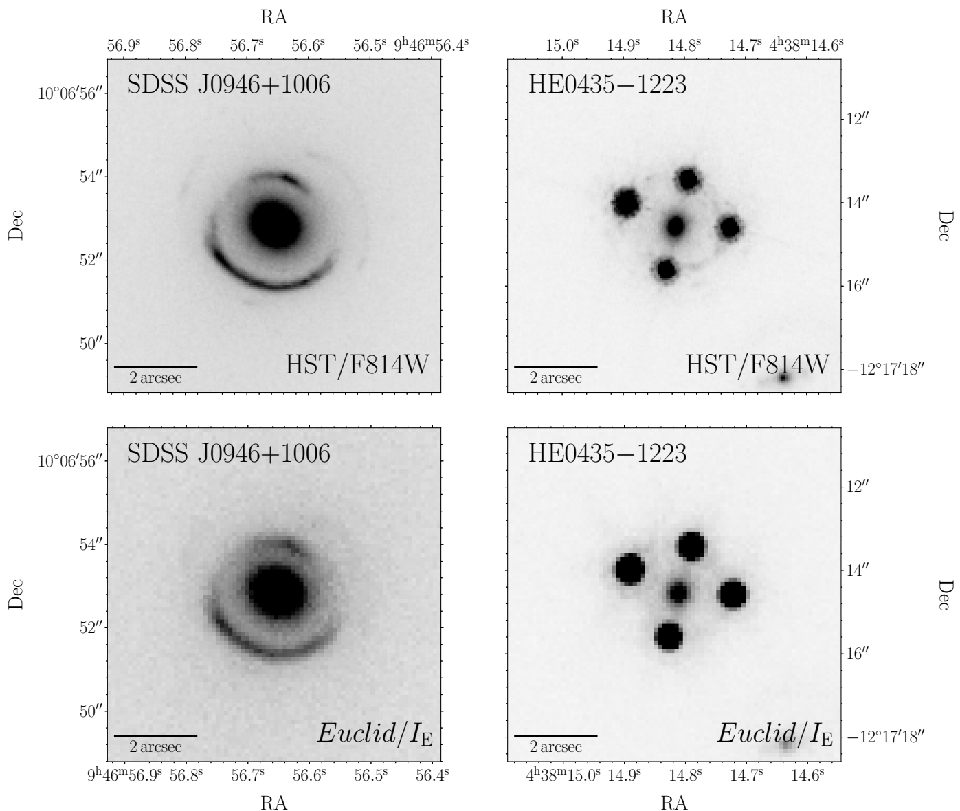
Fig. 11. Examples of simulated Euclid images of galaxy-galaxy strong lensing systems as observed during the Euclid wide survey. In the upper panels, we show the two HST images used to generate the simulations in the lower panels. The system on the left, identified as SDSS J0946+1006 (also known as the Jackpot lens), consists of a double Einstein ring lensed by a galaxy at z = 0.222 (at the centre of the image). The HE0435–1223 system on the right is a quadruple imaged quasi-stellar object (QSO) at z = 1.693 lensed by a galaxy at z = 0.455 .
