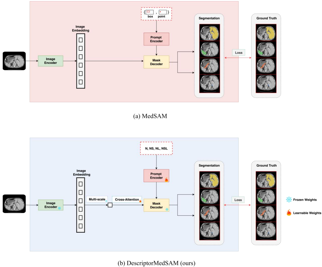
Figure. 1 Comparison between (a) MedSAM and (b) DescriptorMedSAM.
