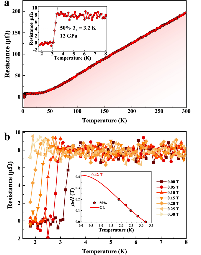
FIG. 4. a Electrical transport measurements of the synthesized hydride under 12 GPa. b Temperature dependence of the electrical resistance under applied magnetic fields of \mu_0 H = 0-0.3 T at 12 GPa. Inset: Upper critical field versus temperature following the criterion of 50% of the resistance in the metallic state at 12 GPa, fitted with the GL model [80].
