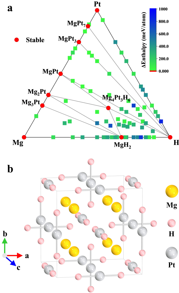
FIG. 1. a Ternary phase diagram of the Mg–Pt–H system at ambient pressure based on DFT calculations. Various structures, represented by squares, are colored according to their distance from the convex hull, with red solid circles representing thermodynamically stable structures. Fm\bar{3}m Pt, P6_3/mmc Mg, and Pa\bar{3} H 2 were used as elemental ground-state structures. b The crystal structure of Im\bar{3}m Mg 4 Pt 3 H 6 . Mg, Pt and H atoms are shown as yellow, gray and pink spheres, respectively.
