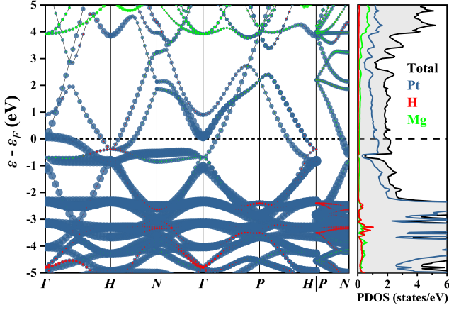
FIG. 3. Electronic band structure (left panel) and projected DOS (right panel) of Im\bar{3}m Mg_4Pt_3H_6 at ambient pressure. Point sizes indicate the respective projected weight and the dotted horizontal line represents the Fermi level.
