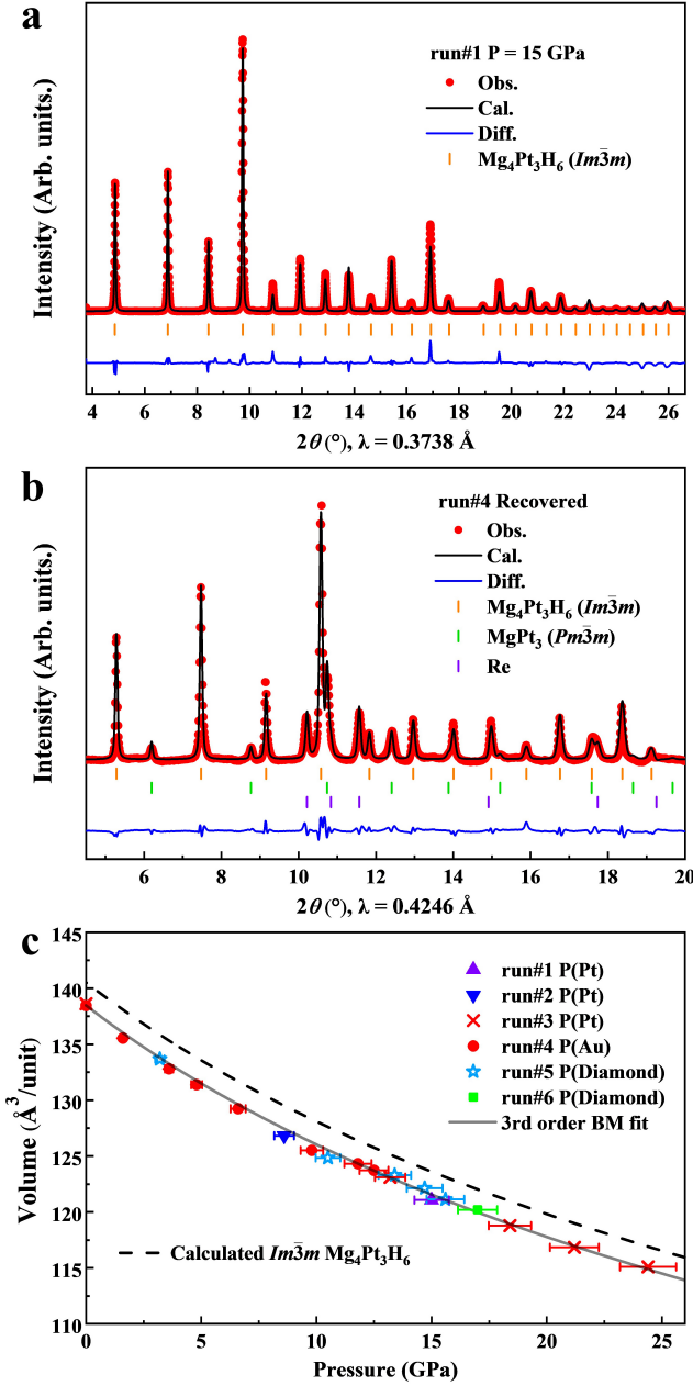
FIG. 2. a Representative synchrotron powder XRD pattern (red points) for a sample synthesized at 15 GPa (measured at room temperature) with Rietveld refinement ( R_{wp} = 1.46\% and R_p = 2.83\% ) of the predicted Im\bar{3}m Mg_4Pt_3H_6 structure (black line). The blue line shows the Rietveld residual and vertical ticks marks indicate allowed Bragg reflections. b Rietveld refinement ( R_{wp} = 2.48\% and R_p = 1.53\% ) of the experimental XRD data at ambient pressure. Impurity peaks from Pm\bar{3}m - MgPt_3 and the Re gasket are represented by green and purple ticks, respectively. c Pressure-Volume data for Im\bar{3}m Mg_4Pt_3H_6 obtained from all runs during decompression. The solid and dashed lines represent the experimental and DFT-PBE equations of state, respectively, as determined using the 3rd-order Birch-Murnaghan equation. Pressure markers for different experimental runs are indicated.
