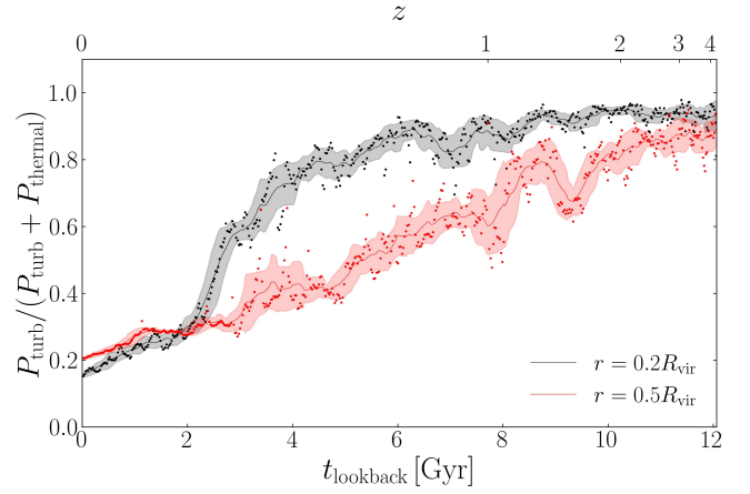
Figure 4. Evolution of the ratio of turbulent pressure ( P_{\text{turb}} ) to total pressure ( P_{\text{turb}} + P_{\text{thermal}} ) in the CGM of the FIRE m12i simulation. Different colors denote gas at r = 0.2 R_{\text{vir}} (black) and at r = 0.5 R_{\text{vir}} (red). Dots represent individual data points, while lines and shaded bands represent running averages and dispersions within a 600 Myr window. The inner CGM exhibits a relatively sharp transition (within \approx 2 Gyr) between turbulent pressure dominance to thermal pressure dominance, corresponding to the formation of a quasi-static hot phase in the inner CGM as seen in Fig. 3. At larger radii the importance of turbulence decreases more gradually with time.
