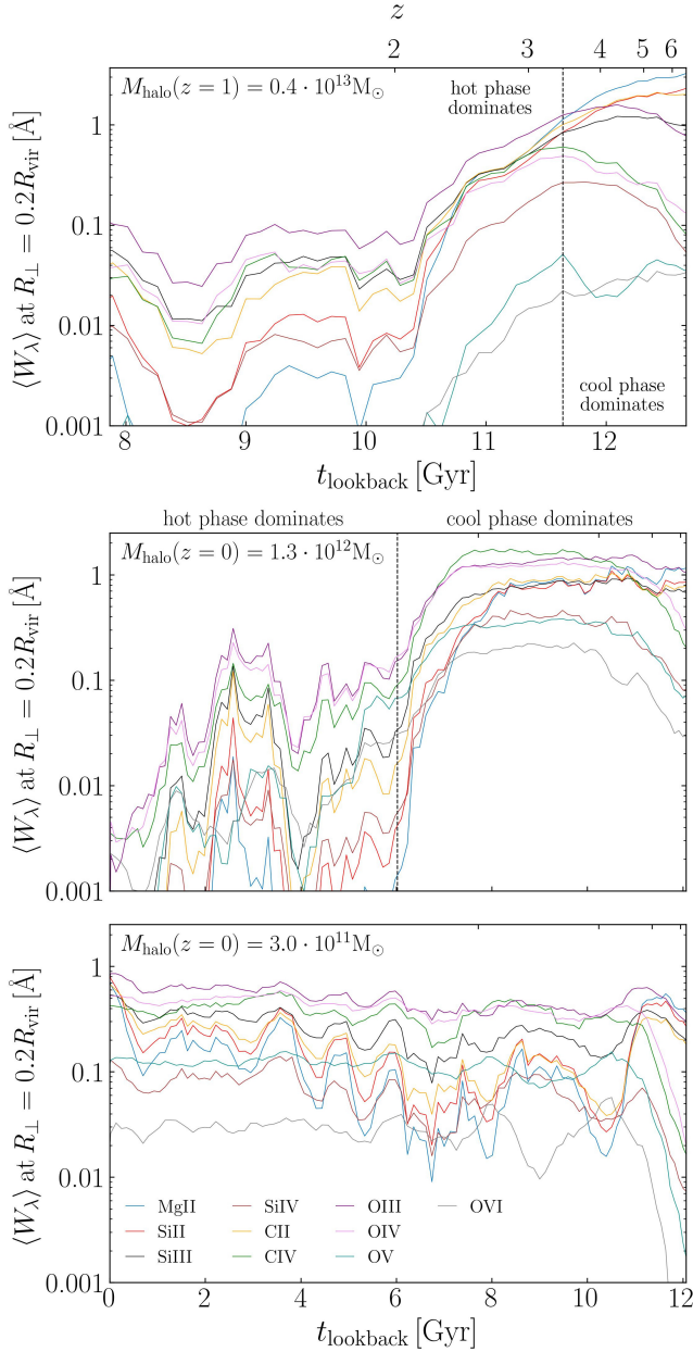
Figure 9. Evolution of mean W_\lambda at R_\perp = 0.2R_{\text{vir}} for the three simulations shown in Fig. 8. The dashed vertical lines indicate the transition from an inner CGM dominated by cool gas and turbulence to an inner CGM dominated by the hot phase. Equivalent widths are high ( \approx 1 \text{ \AA} ) before the transition and decrease afterward. The lowest-mass halo shown in the bottom panel remains cool and turbulent at all times, with 0.1 < W_\lambda < 1 \text{ \AA} for all ions except O VI.
