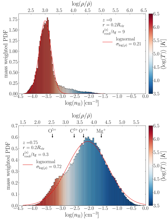
Figure 2. Density distribution of gas in a thin shell with r = 0.2R_{\text{vir}} , for the two snapshots shown in Fig. 1. Color indicates the mean temperature at each density, and the top axes denote the density in units of the cosmic mean. The ratio of hot gas cooling time to free-fall time is noted in the panels. At z = 0 (top) the distribution is narrow with \sigma_{\log \rho} = 0.21 and a tail towards high densities, as expected in the common CGM paradigm with a low density hot phase and denser cool clouds. Conversely, at z = 0.75 (bottom) the gas is predominantly cool and the distribution is a broad lognormal with \sigma_{\log \rho} = 0.72 , as expected in isothermal turbulent gas with Mach \sim 10 . Labels denote the median density of gas which produces each ion.
