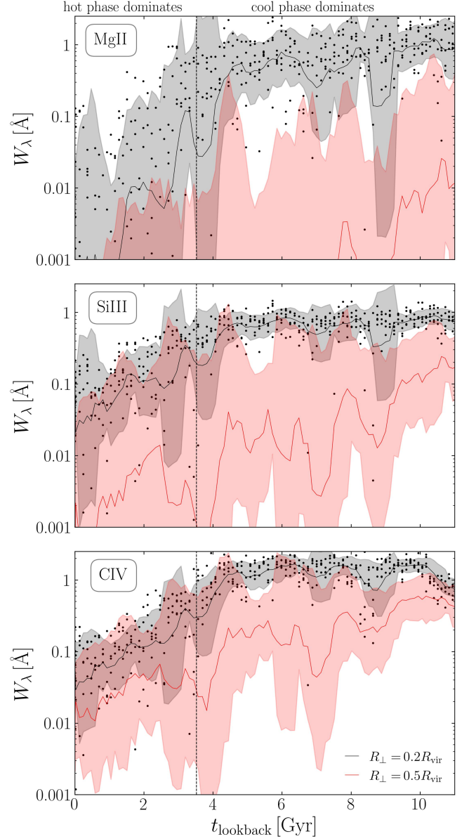
Figure 6. Predicted evolution of CGM absorption equivalent widths in m12i. Different panels show different ions, while impact parameters are denoted by color. Dots represent individual mock sightlines (shown for R_\perp = 0.2 R_{\text{vir}} ), while lines and bands represent averages and dispersions within a running 600 Myr window. Vertical lines denote the time after which the hot phase dominates (see Fig. 3). At t_{\text{lookback}} > 4 \text{ Gyr} when the cool phase dominates we predict W_\lambda(0.2 R_{\text{vir}}) \approx 1 \text{ Å} in all ions, consistent with the analytic approximation (eqn. 13). After the hot phase forms W_\lambda(0.2 R_{\text{vir}}) \ll 1 \text{ Å} .
