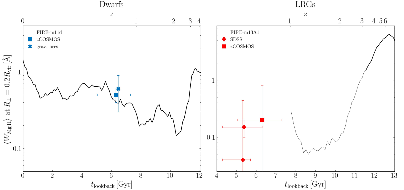
Figure 11. Observed Mg II absorption in dwarf galaxies (left) and in LRGs (right) versus FIRE predictions. Solid lines show predicted \langle W_{2796+2803} \rangle at R_{\perp} = 0.2R_{\text{vir}} , with thicker segments corresponding to pre-ICV ( f_{\text{cool}} > 0.5 , turbulence-dominated) times. m11d remains turbulence-dominated down to z = 0 . Observed values from the surveys listed in Table 3 are plotted as markers and errorbars, with marker color indicating star-forming (blue) or quiescent (red) galaxies. Blue dwarf galaxy samples are consistent with a turbulence-dominated inner CGM, while LRG observations suggest thermally supported inner CGM.
