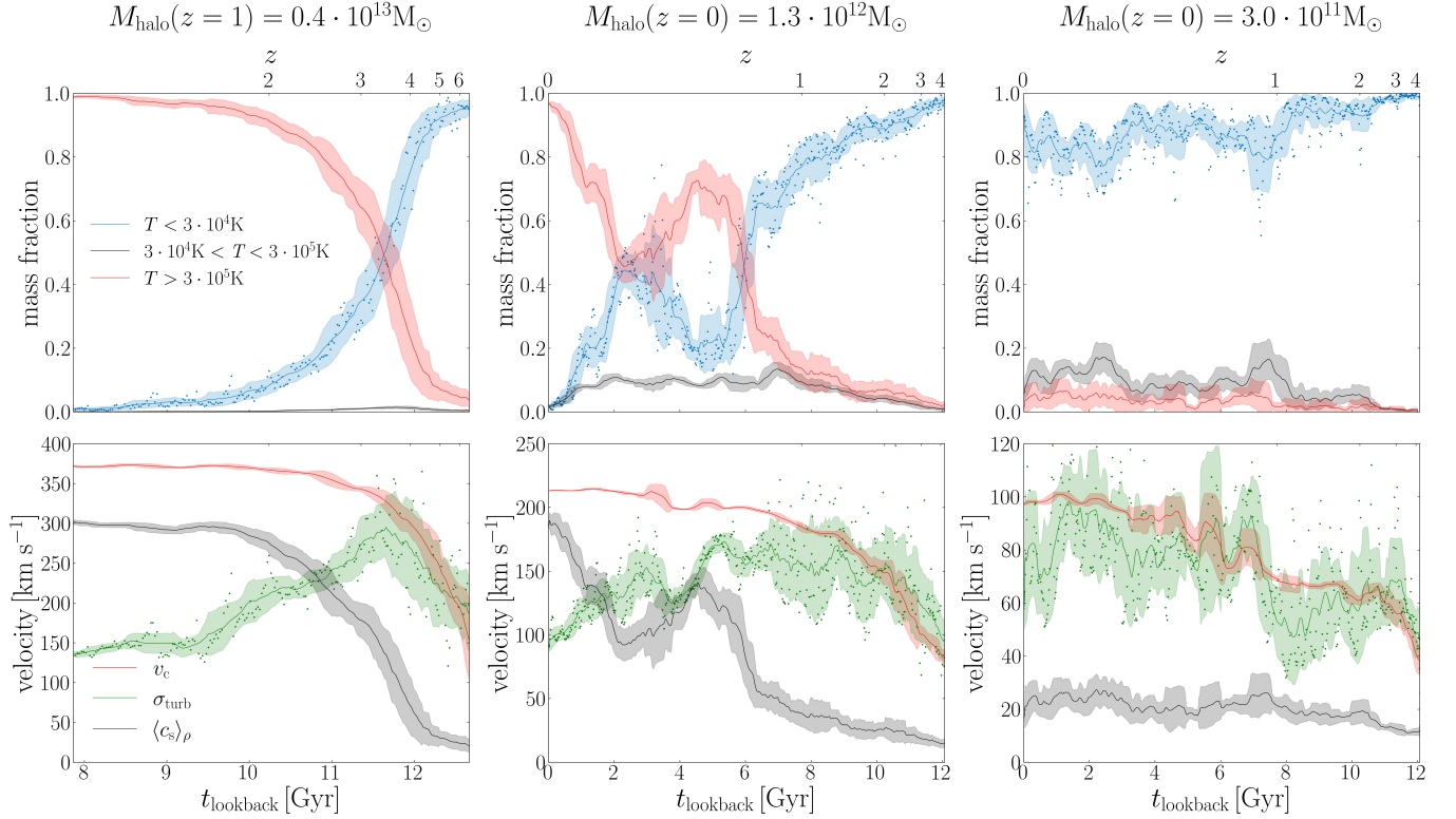
Figure 8. (Top:) Evolution of the mass fractions of different CGM phases at r = 0.2R_{\text{vir}} , in three FIRE simulations of halos of different masses. The panels from left to right correspond to a group-size halo (‘m13A1’), a Milky Way-mass galaxy (‘m12b’), and a dwarf galaxy (‘m11d’). Dots represent individual snapshots (shown only for the cool phase for clarity), while lines and bands represent averages and dispersions within a running 600 Myr window. (Bottom:) Evolution of the turbulent velocity (green), circular velocity (red), and mass-weighted sound speed (black) at r = 0.2R_{\text{vir}} . Note the difference in plotted velocity ranges between the panels. A significant increase in hot gas mass fraction is apparent around t_{\text{lookback}} \approx 7 Gyr in m12b and t_{\text{lookback}} \approx 12 Gyr in m13A1, indicating the formation of a quasi-static hot phase with subsonic turbulence. The short-term decrease in hot gas mass fraction in m12b at t_{\text{lookback}} \approx 2 Gyr is associated with a major merger. The m11d galaxy on the right remains dominated by the supersonically turbulent cool phase at all times.
