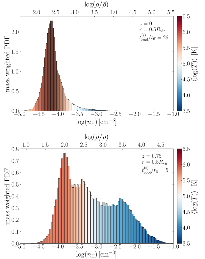
Figure A1. Similar to Fig. 2, for r = 0.5 R_{\text{vir}} . Panels show mass-weighted gas density distributions in a thin shell in the m12i simulation at z = 0 (top) and at z = 0.75 (bottom). Color indicates average temperature at each density bin. In both snapshots hot gas dominates the mass consistent with t_{\text{cool}}^{(s)} > t_{\text{ff}} (noted), though with a significantly more prominent cool gas phase at z = 0.75 .
