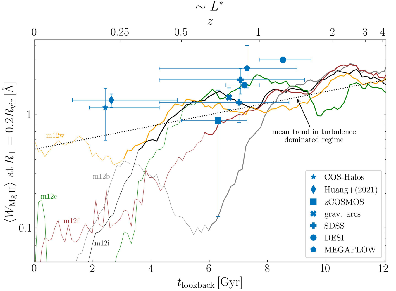
Figure 10. Observed Mg II absorption at R_{\perp} = 0.2R_{\text{vir}} from blue \sim L^* galaxies versus FIRE predictions. Solid colored lines show the evolution of the mean Mg II equivalent width \langle W_{2796} + W_{2803} \rangle in five simulated \sim L^* galaxies. Thicker segments of each curve indicate pre-ICV ( f_{\text{cool}} > 0.5 , turbulence-dominated) times, and the dotted black line shows the mean trend in this regime. Thin segments show post-ICV ( f_{\text{cool}} < 0.5 , thermally-supported) times which in most cases predict substantially lower \langle W_{\text{MgII}} \rangle . Observed values from the blue \sim L^* surveys listed in Table 3 are plotted as markers and errorbars. Observed \langle W_{\text{MgII}} \rangle at R_{\perp} = 0.2R_{\text{vir}} in star-forming \sim L^* galaxies are consistent with the predictions of turbulence-dominated inner CGM to a factor of \approx 2 .
