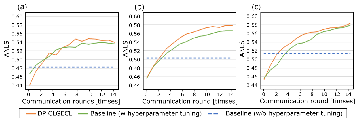
Figure A.5: convergence curve evaluating using the global model. (a) validation ANLS at \varepsilon = 1 , (b) validation ANLS at \varepsilon = 4 , (c) validation ANLS at \varepsilon = 8 . We used clipping radius S = 0.5 , the number of client sampling C = 2 , the learning rate \eta = 0.0002 , and the number of communication round R = 14 for hyperparameter selection.
