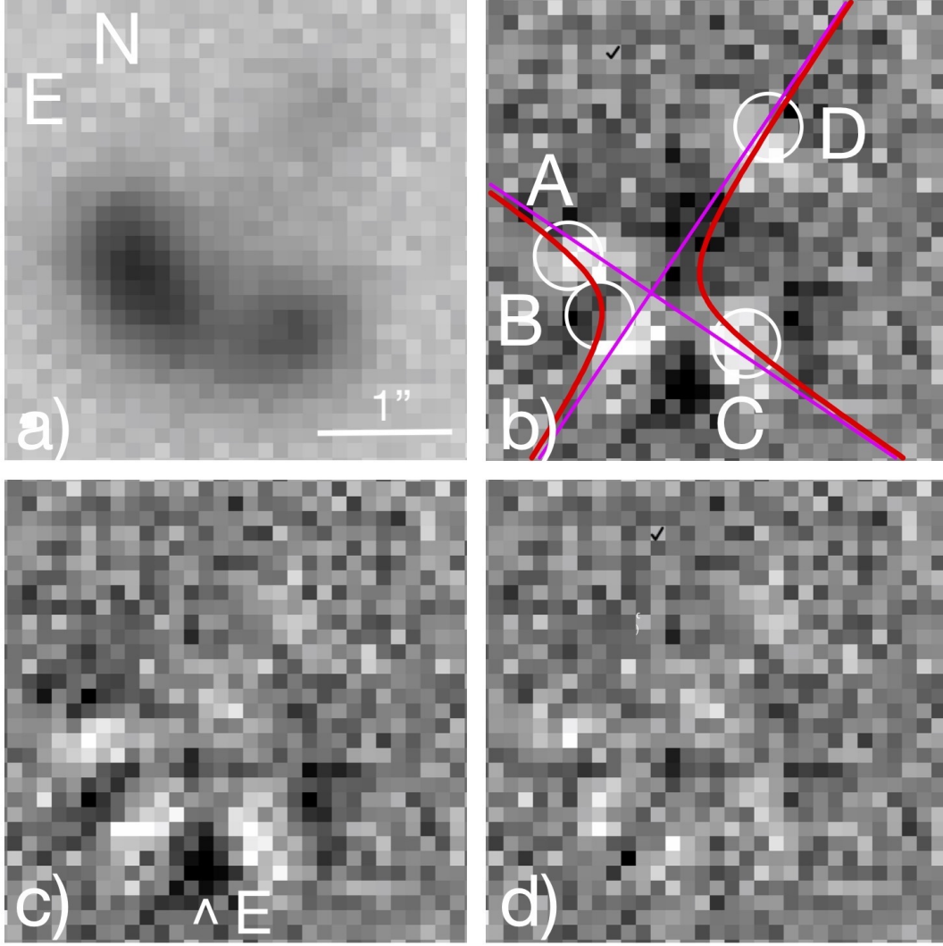
Figure 3. (a) DELQQ 1258–0319 observed with a Sloan g filter for 900s with the IMACS f/4 camera on the Magellan Baade telescope. A negative grayscale is used to highlight the low surface brightness of the central lens, which is substantially fainter than the four images surrounding it. (b) Four point sources, A , B , C & D , have been fitted and subtracted. A rectangular hyperbola (red) has been drawn through the fitted positions. According to Witt (1996), if the potential is elliptical, the hyperbola’s asymptotes (magenta) are parallel to its major and minor axes and the lensing galaxy must lie on the longer, primary branch of the hyperbola. A faint source, that we take to be the lensing galaxy, is consistent with Witt’s prediction. (c) A point source has been fitted to the lensing galaxy, which is too faint to permit determination of its extent. White regions indicate oversubtraction of the point sources. (d) A substantial residual southeast of image C , which we call E , has been fitted by a point source and subtracted. The positions from this fit are shown in panel (b) as white circles.
