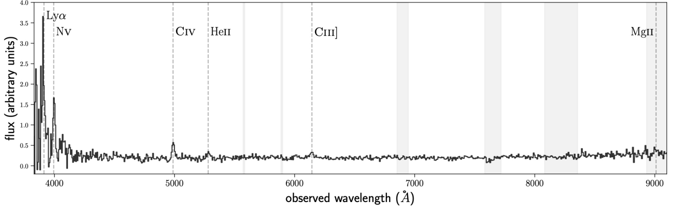
Figure 2. NOT spectrum of the brightest quasar component A , extending from 3800 to 9000 Å. The high ionization lines of N V, C IV and He II seen at z = 2.225 are narrow, with widths ranging from 1300-2000 km/s, suggesting a Type 2 AGN rather than a quasar.
