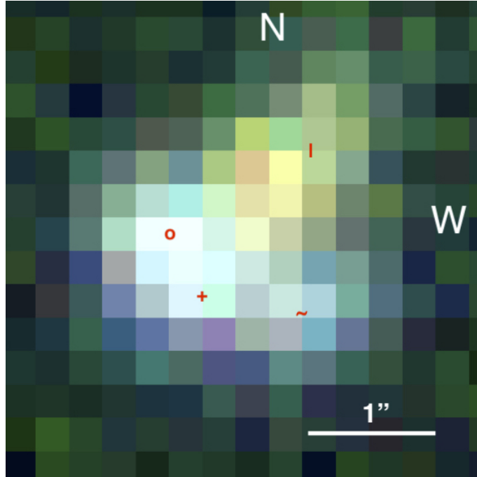
Figure 1. A color composite representation of DELQQ 1258–0319 taken with DECam on the Blanco Telescope, using DES r, i , and z exposures (for blue, green and red) taken as part of the DELVE survey. The approximate positions of four images subsequently labelled A, B, C , and D are shown in red with the symbols \circ, +, \sim , and | , respectively.
