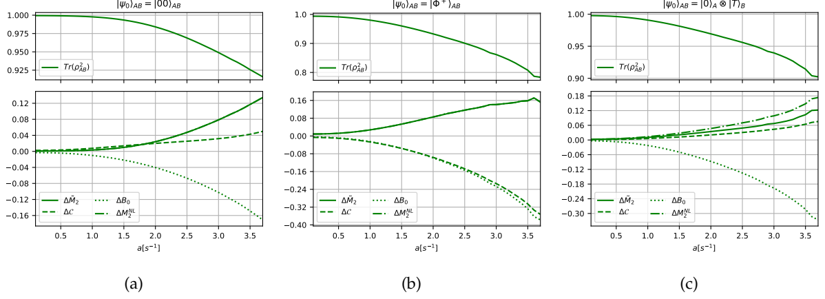
Figure 7: Plots of the harvested magic (local and non local) and entanglement, together with the expectation value of the Bell operator, as a function of the acceleration a_{\perp} in the case of perpendicular acceleration. Panel 7a shows the evolution of the harvested resources when the detectors start in the state |\psi_0\rangle_{AB} = |00\rangle_{AB} . Panel 7b shows the harvested resources when the detectors start in the Bell state |\Phi^+\rangle_{AB} . Panel 7c shows the harvested resources when the detectors are initialized in the state |\psi_0\rangle_{AB} = |0\rangle_A \otimes |T\rangle_B . The upper plots show the evolution of the purity of the state of the detectors.
