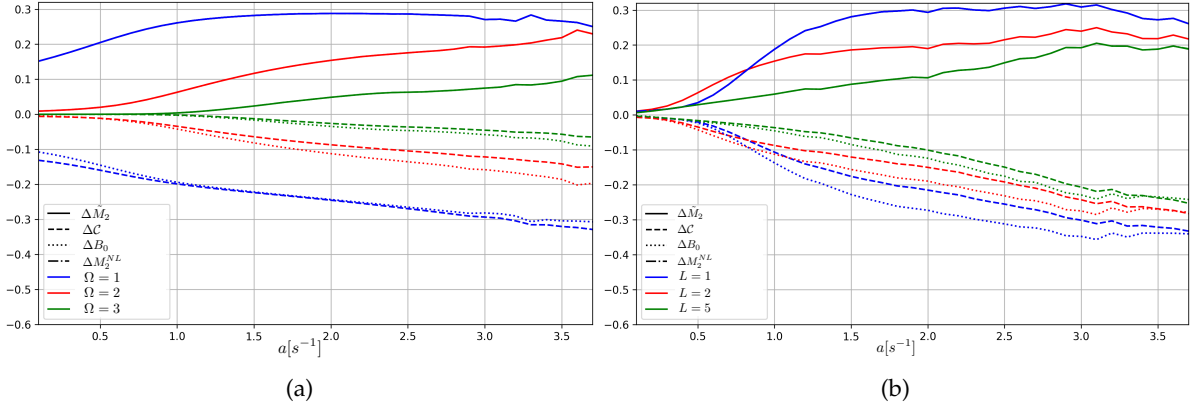
Figure 5: Plot of the variation of the non-stabilizerness, concurrence, expectation value of the Bell operator and non-local non-stabilizerness as a function of the acceleration when the detectors are initialized in the maximally entangled state \rho_{AB}(0) = |\Phi^+\rangle\langle\Phi^+| for different values of the detectors frequency. In the plot we have set \sigma = 1 and L = 1 . Different line shapes represent the various quantities, while different colours represent different values of \Omega , as in the legend. From a qualitative point of view, one can once again observe that all the harvested non-stabilizerness is non-local. This feature, as explained in the main text, is the one responsible for the non violation of the CHSH inequality. The only difference with respect to the scenario where the detectors are initialized in the state |00\rangle\langle 00| is that the SRE also depends on the initial separation L . However, there are no choice of parameters for which the CHSH inequality is violated.
