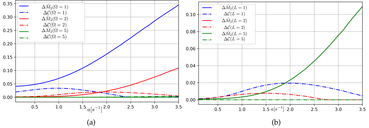
Figure 3: Variations of SRE \tilde{M}_2(\rho_{AB}) (solid line) and concurrence \Delta\mathcal{C}(\rho_{AB}) (dashed line), as a function of the (parallel) acceleration a_{\parallel} , for various choices of parameters, with the detectors initialized in the state \rho_{AB} = |00\rangle\langle 00| . In Fig. 3a we study the two resources for different values of \Omega , setting \sigma = 1 and L = 1 . Notice that for \Omega = 1 , for a = 0 one has a non zero SRE, in agreement with the observation made in the inertial setting. One can also notice that the harvested SRE becomes larger for lower values of \Omega .
