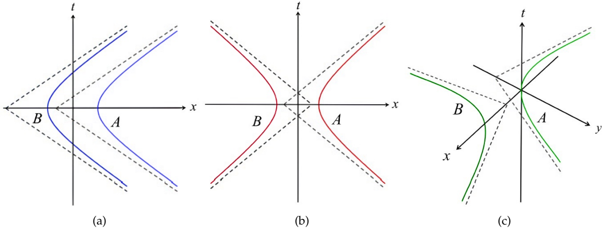
Figure 1: Trajectories of accelerated UDW detectors: (a) detectors with parallel acceleration a_{\parallel} ; (b) detectors with antiparallel acceleration a_{\parallel} ; (c) detectors with perpendicular acceleration a_{\perp} .
