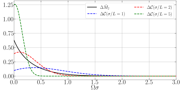
Figure 2: Plot of the SRE as a function of \Omega\sigma and of the concurrence for different values of \sigma/L . The initial state of the detectors is \rho_{AB} = |00\rangle\langle 00| . For small values of the product \Omega\sigma one can see that the final state of the detectors has significant amount of non-stabilizerness. While this is in contrast with the vacuum state of the field being a stabilizer state (i.e. SRE-free state), the presence of SRE is explained by noticing that the interaction between the detectors and the field is non-Clifford, such that some non-stabilizerness is introduced in the system for small values of \sigma\Omega . On the other hand, for \Omega\sigma \gtrsim 1 , one can get rid of this spurious contribution and genuinely harvest SRE from the field.
