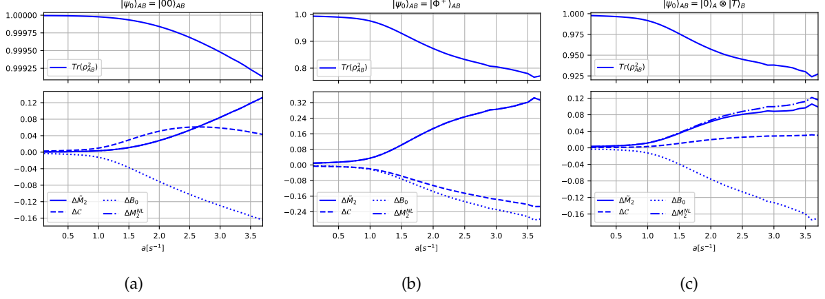
Figure 4: Variations of SRE \Delta\tilde{M}_2(\rho_{AB}) (solid line), concurrence \Delta C(\rho_{AB}) (dashed line), non-local SRE \Delta M_2^{NL}(\rho_{AB}) (dashed-dotted line) and value of Bell operator \Delta B_0 (dotted line) as a function of the (parallel) acceleration a_{\parallel} , together with the corresponding purity of the state (see upper plots). Panels (a) Initial state |00\rangle , (b) initial state |\Phi^+\rangle , (c) initial state |0\rangle_A \otimes |T\rangle_B . In panel (a) and (b) the curves for \Delta\tilde{M}_2(\rho_{AB}) and \Delta M_2^{NL}(\rho_{AB}) overlap perfectly as all the harvested SRE is non-local. Notice that the state of the detectors, for the initial state |\psi_0\rangle_{AB} = |00\rangle , is always pure with very good approximation.
