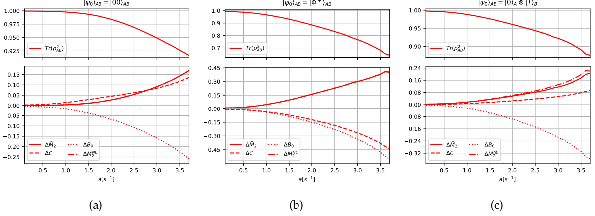
Figure 6: Plots of the harvested magic (local and non local) and entanglement, together with the expectation value of the Bell operator, as a function of the acceleration a in the case of antiparallel acceleration a_{\parallel} . Panel 6a shows the evolution of the harvested resources when the detectors start in the state |\psi_0\rangle_{AB} = |00\rangle_{AB} . Panel 6b shows the harvested resources when the detectors start in the Bell state |\Phi^+\rangle_{AB} . Panel 6c shows the harvested resources when the detectors are initialized in the state |\psi_0\rangle_{AB} = |0\rangle_A \otimes |T\rangle_B . The upper plots show the evolution of the purity of the state of the detectors.
