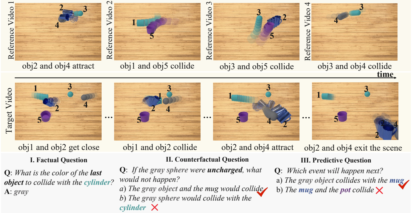
Fig. 7: Qualitative examples of more diverse scenes in the ComPhy-DIV. As shown in the figure, we have more diverse physical interactions between the blue mug and the sphere in the video. The image background is also more diverse with different textures and colors in contrast to the original ComPhy in [8].
