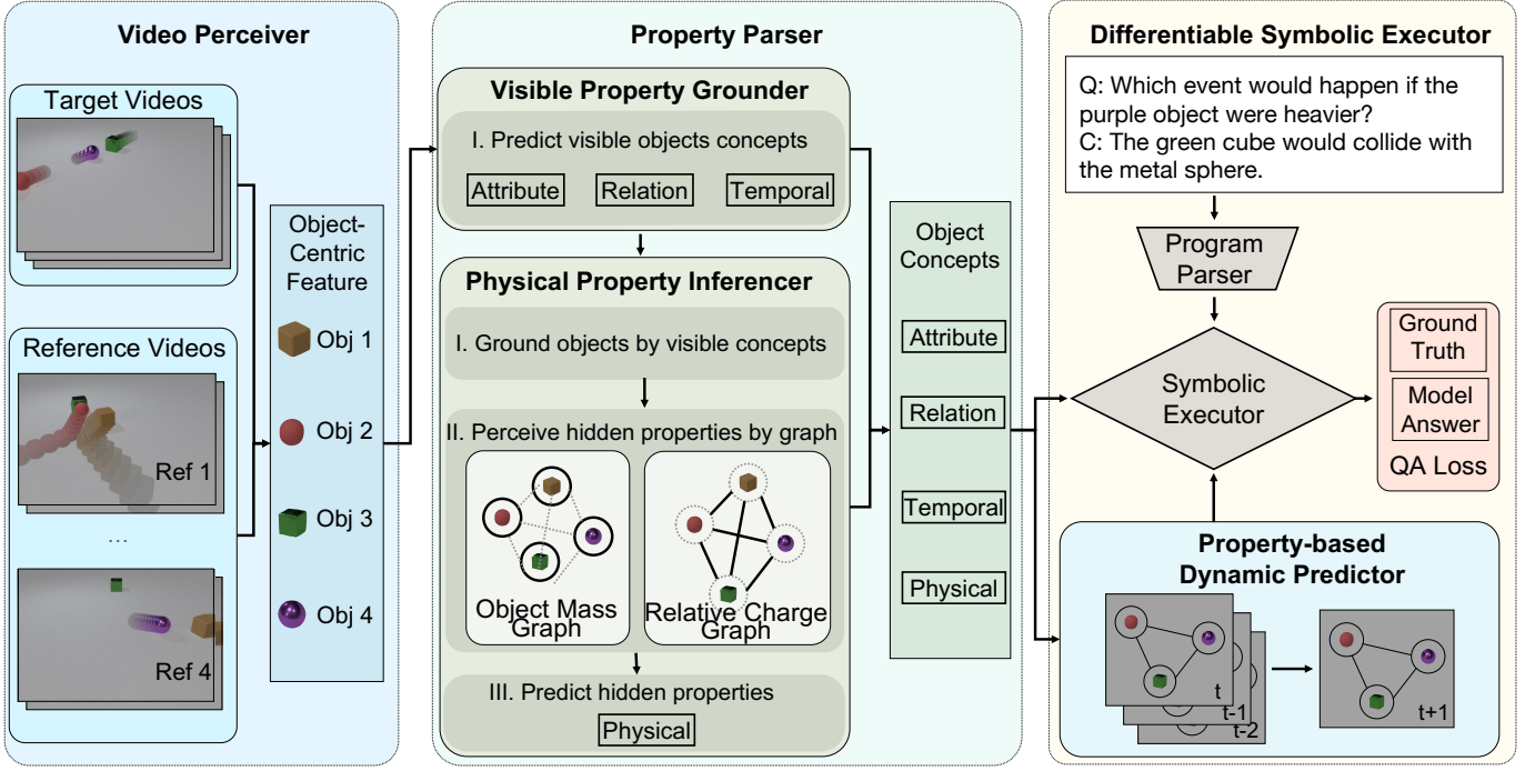
Fig. 4: The perception module detects objects’ location and visual appearance attributes. The physical property learner learns objects’ properties based on detected object trajectories. The dynamic predictor predicts objects’ dynamics in the counterfactual scene based on objects’ properties and locations. Finally, an execution engine runs the program parsed by the language parser on the predicted dynamic scene to answer the question.
