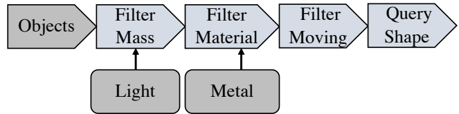
Fig. 23: Sample of factual questions and their underlying functional programs in ComPhy.
