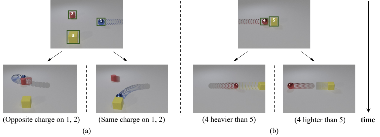
Fig. 1: Non-visual properties like mass and charge govern the interaction between objects and lead to different motion trajectories. a) Objects attract and repel each other according to the (sign of) charge they carry. b) Mass determines how much an object’s trajectory is perturbed during an interaction. Heavier objects have more stable motion.
