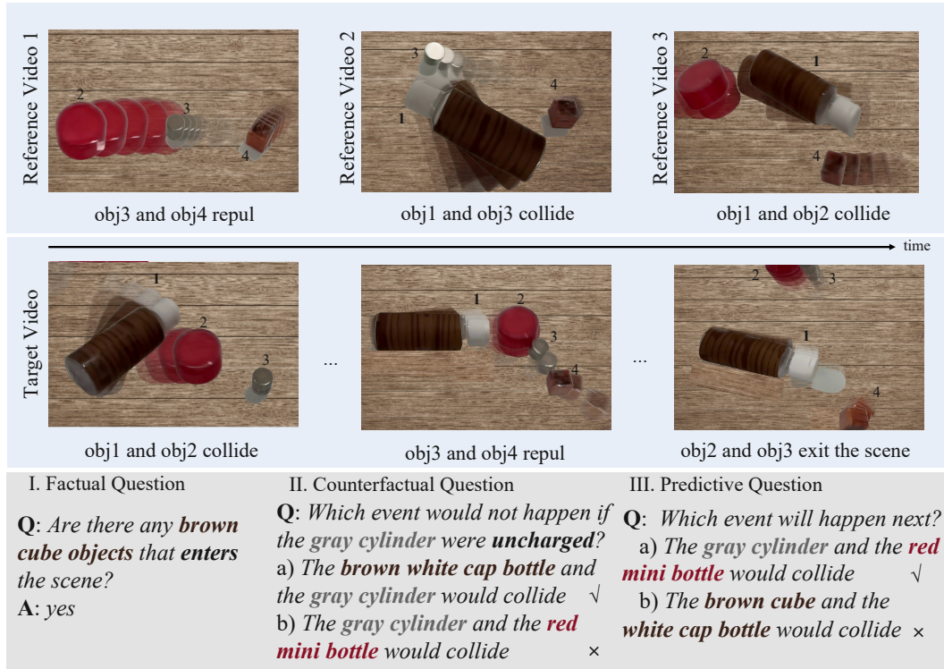
Fig. 19: More qualitative examples of more diverse scenes in the ComPhy-REAL.
