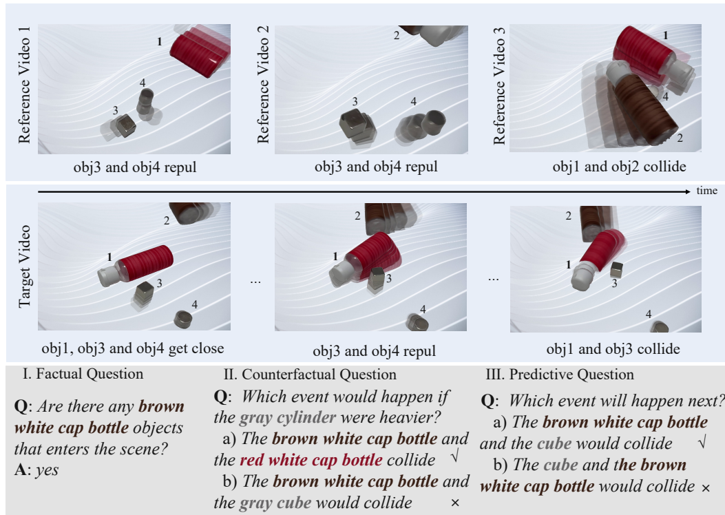
Fig. 20: More qualitative examples of more diverse scenes in the ComPhy-REAL.
