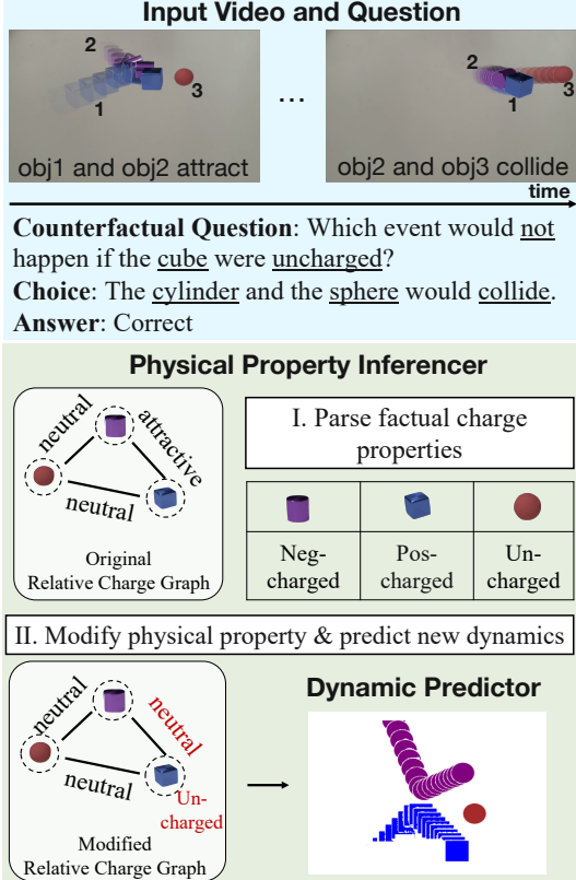
Fig. 5: A qualitative example of PCR on ComPhy. The left-up blue box shows the original video and a counterfactual question to answer. The right half table shows the executable program sequence parsed from the question with concepts related to it and outputs after execution. Specifically, the left-down chart illustrates the execution process of PCR for the program “counterfact charge”: 1. PCR utilizes a PPI to parse factual charge properties of objects in the scene; 2. PCR modifies their properties according to the counterfactual concept and predicts new dynamics using a dynamic predictor.
