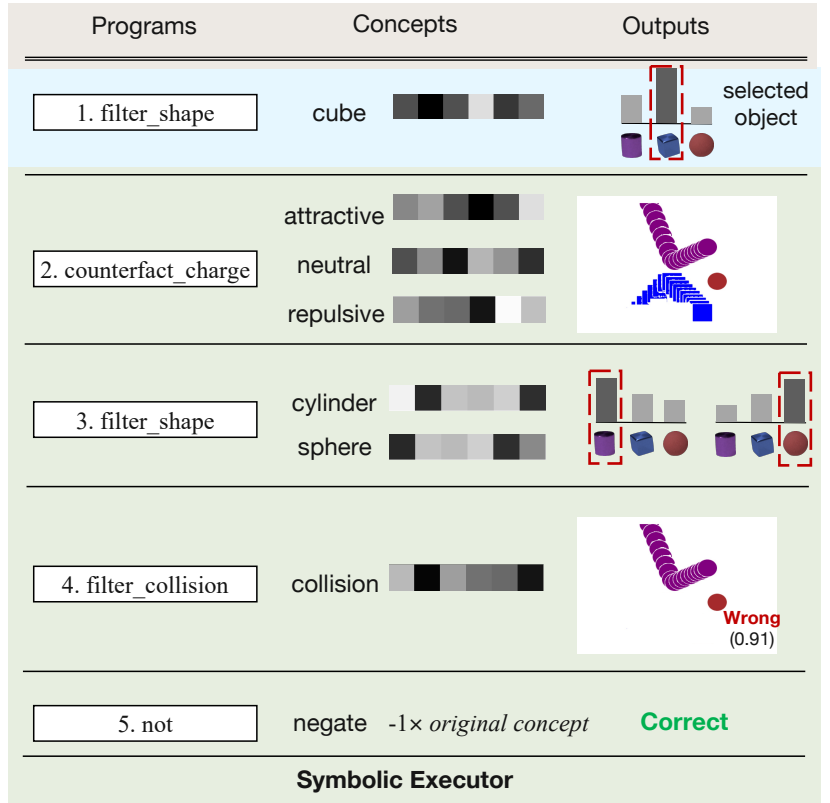
Fig. 5: A qualitative example of PCR on ComPhy. The left-up blue box shows the original video and a counterfactual question to answer. The right half table shows the executable program sequence parsed from the question with concepts related to it and outputs after execution. Specifically, the left-down chart illustrates the execution process of PCR for the program “counterfact charge”: 1. PCR utilizes a PPI to parse factual charge properties of objects in the scene; 2. PCR modifies their properties according to the counterfactual concept and predicts new dynamics using a dynamic predictor.
