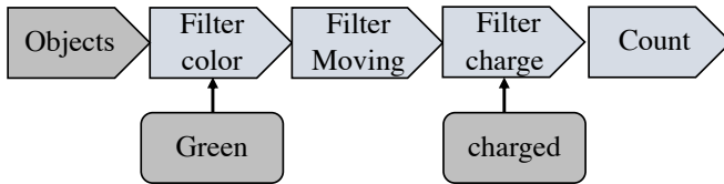
Fig. 23: Sample of factual questions and their underlying functional programs in ComPhy.
