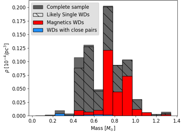
Figure 6. Mass distribution for our Complete sample corrected by the 1/V_{max} volume. The red and blue bins represent the WDs with magnetic field and with close pairs, respectively. The hatch-filled bins indicated the Likely single WDs .
