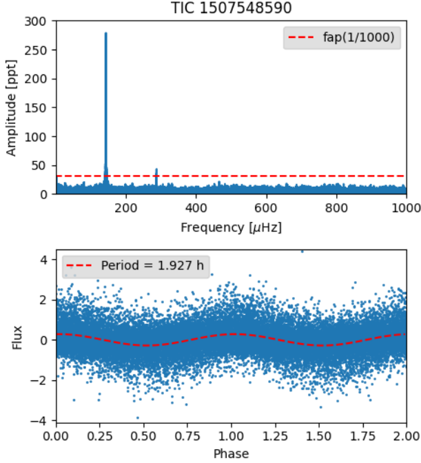
Figure 2. Time series analysis for the star TIC 1507548590. The top panel shows the Fourier Transform as well as its 1/1000 false alarm probability (red dashed line). The bottom panel shows the light curve folded on the period of 1.9272 hours and a sinusoidal curve with the same period in red.
