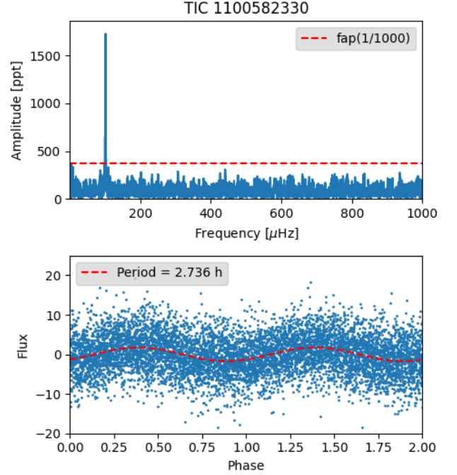
Figure 3. Time series analysis for the star TIC 1100582330. The top panel shows its Fourier Transform as well as its 1/1000 false alarm probability (red dashed line). The bottom panel shows the light curve folded on the period of 2.736 hours and a sinusoidal curve with the same period in red.
