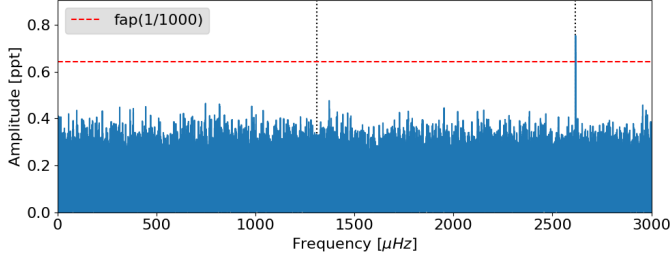
Figure 9. Fourier Transform of TESS data of star TIC 262548040. The horizontal red line indicates the false alarm probability FAP=1/1000 and the vertical dotted lines indicate the peak of 0.106 h and its double.
