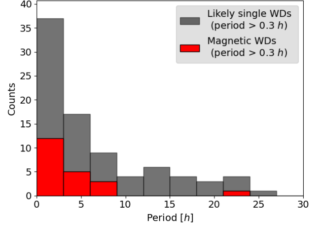
Figure 8. Rotational period distribution up to 30 h for the Likely single WDs excluding periods shorter than 0.3 h. The red bins indicate the magnetic stars of the sample.
