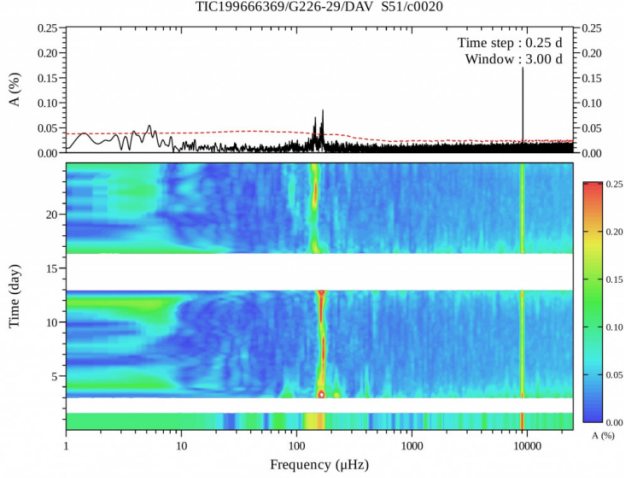
Figure 12. Running Fourier transform of G226-29 20 s data from sector 51. The tall peak on the right is the pulsation triplet around 109 s, while the region around 200 \mu Hz corresponds to the peaks around 4500 s.
