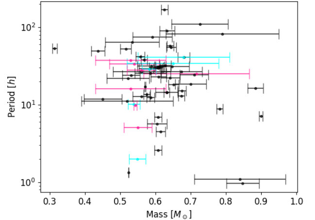
Figure 1. Rotation period versus mass relation, for period determinations from asteroseismology. The period axis is in log scale. Black, cyan, and pink dots indicate DAV, DBV, and DOV stars respectively.
