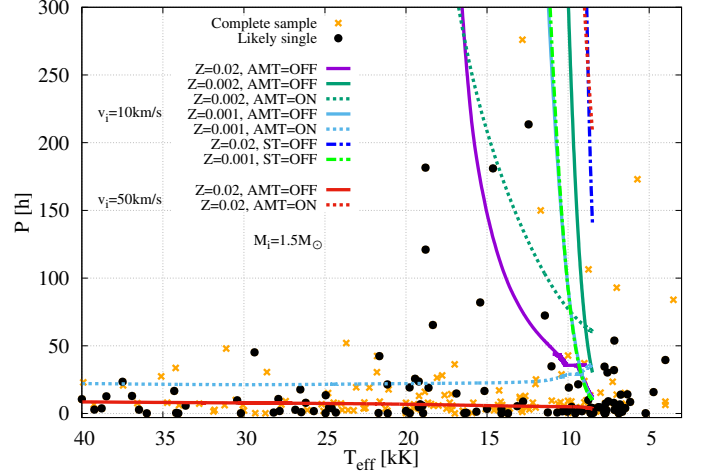
Figure 14. Observational data of the surface rotation of white dwarf stars (orange crosses for the complete sample and black dots for the likely single sample
