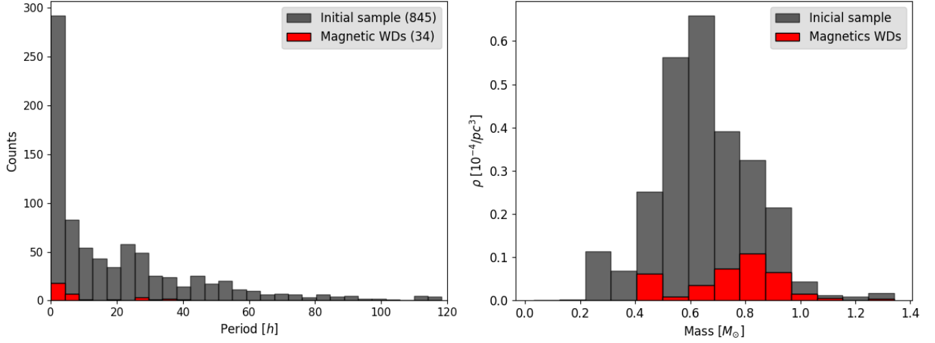
Figure 17. Mass distribution for our Initial corrected by the 1/V_{max} volume.
