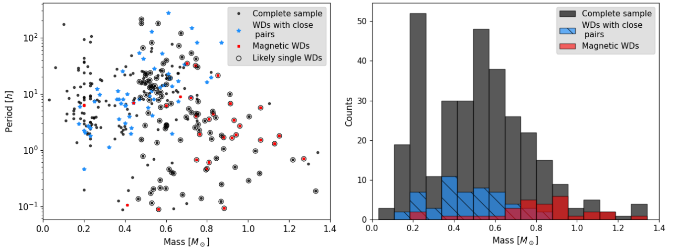
Figure 5. The left panel displays the rotational period in hours in log scale versus mass in solar masses, while the right panel shows the mass distribution of sample 1. The red and blue dots/bins represent the WDs with magnetic field and with close pairs detected
