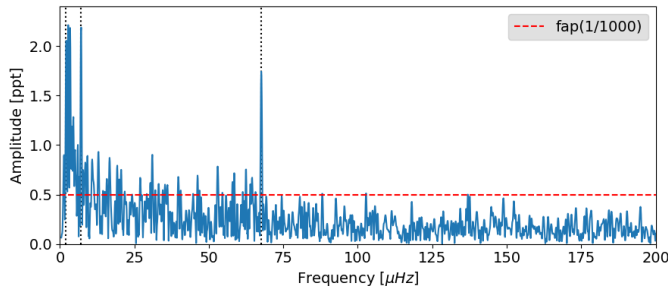
Figure 10. Fourier transform of NGC 1501 data at low frequencies.
