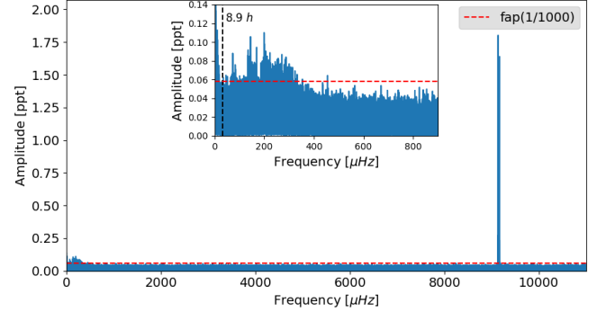
Figure 13. Fourier transform of the 20 s data for G226-29 from sectors 40 to 41 and 47 to 60. The inset plot zooms the FT at low frequencies. The red dashed line indicates the false alarm probability. The large peak on the right is the pulsation triplet at 109.47235s@1.81mma, 109.27929s@0.57mma, 109.08690s@1.62mma, while the region around 200 \mu Hz corresponds to the wandering peak around 4500 s.
