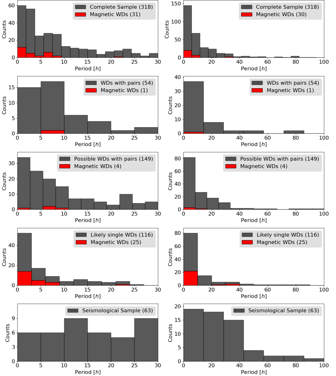
Figure 7. Variability period histograms for different samples of this work over and, last line, histograms of rotation periods from seismology. On the left, we present the histograms of periods up to 30 h, and on the right, the histograms of periods up to 100 h. The red bins show the magnetic population in our samples of WDs. The labels indicate the samples plotted as well as their number.
