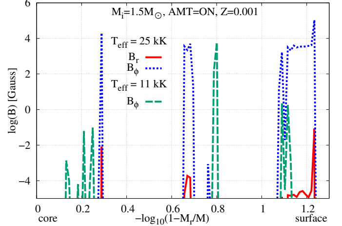
Figure 15. Internal magnetic field at T_{\text{eff}} = 25000 K and 11000 K, generated by the Tayler-Spruit dynamo during the evolution due to differential rotation caused by angular momentum transfer throughout the stellar evolution. B_r is the radial field and B_{\phi} the azimuthal one. The properties of the initial model in the ZAMS are M_i = 1.5 M_{\odot} , Z = 0.001 , and v_i = 10 \text{ km s}^{-1} . For T_{\text{eff}} = 25000 K, the solid red line shows the radial component and the dotted blue line represents the azimuthal one. For T_{\text{eff}} = 11000 K, the dashed green line shows the azimuthal component, and the radial component does not have enough intensity to appear in the plot. The six angular momentum transfer mechanisms operate throughout evolution. Magnetic field values are negligible beyond 1.3 on the x -axis, i.e., towards the surface.
