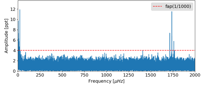
Figure 11. Fourier transform of TIC 7675859 data from sectors 52 to 54.
