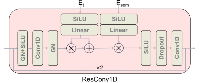
Fig. 2: The ResConv1D module used in our method is conditioned on the time step embedding E_t and the semantic representation E_{sem} .
