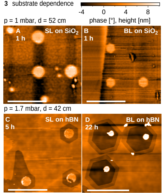
FIG. 3. Substrate dependence of SL/BL graphene (A,B) AFM phase contrast images of a SL (A) and BL (B) section of the same flake on a \text{SiO}_2 substrate, etched for 1 h at T = 450^\circ\text{C} . Round holes of 50 nm diameter were defined before H-etching. AFM topography image of a SL (C) and BL (D) flake on hBN etched for 5 h and 22 h, respectively. Holes of 200 nm (SL) and 100 nm (BL) were defined before etching. For (D) the color scale values are divided by four. The scale bars on all images are 1\ \mu\text{m} .
