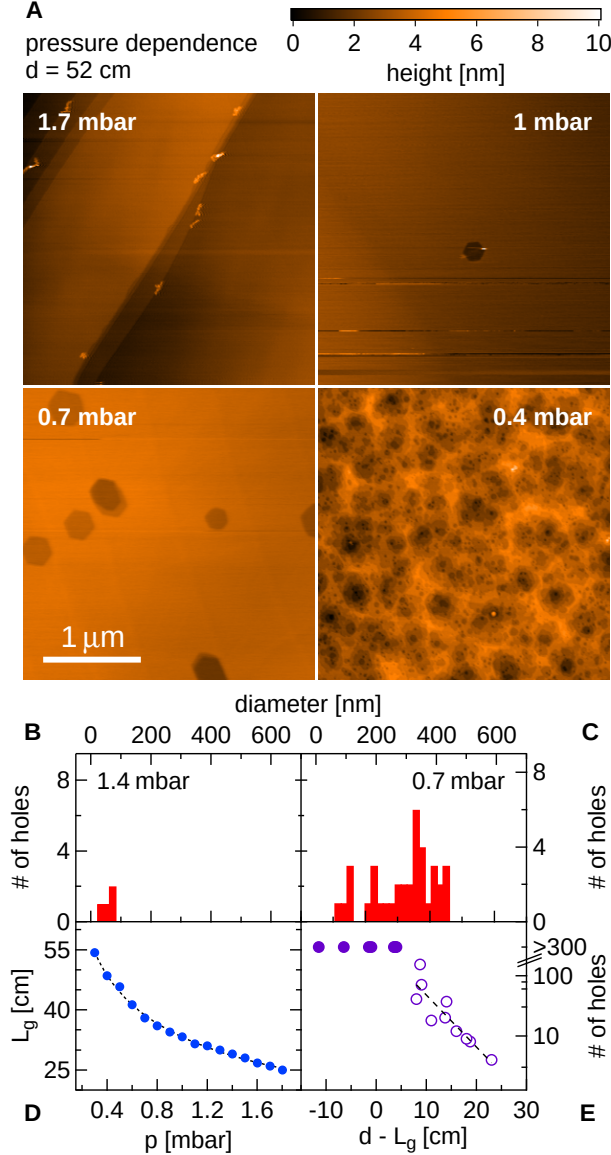
FIG. 2. Pressure dependence of graphite exposures (A) AFM images (tapping mode) of graphite surfaces for various p , as indicated, exposed for one hour at d = 52 cm and T = 400^\circ\text{C} , all shown on the same color scale. All panels are 3 \times 3 \mu\text{m}^2 . (B,C) Histograms from 10 \times 10 \mu\text{m}^2 scans, displaying the number of holes against hole diameter (bin size 20 nm) for p as labeled. (D) Length L_g of the optically visible plasma as a function of p . The dashed curve is a 1/\sqrt{p} fit. (E) Number of holes versus distance from plasma edge d - L_g . A lower bound of 300 holes is given for the heavily etched cases where an exact hole-count was not feasible. The dashed black line is an exponential fit to the data with < 300 holes with 1/e decay length \sim 5 cm.
