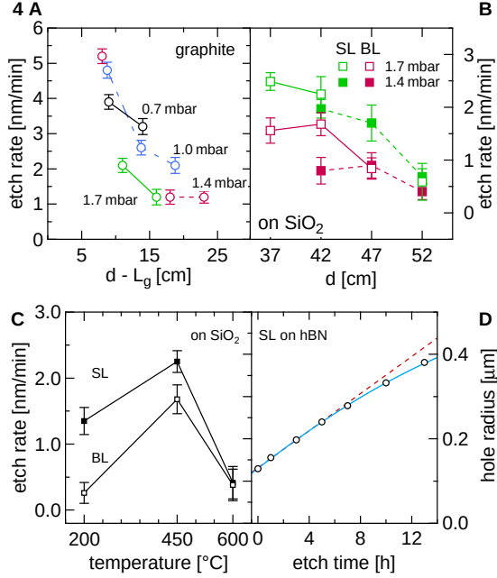
FIG. 4. Anisotropic etch rates (A) Graphite anisotropic etch rate versus distance from plasma d - L_g for several configurations. (B) Etch rate of SL and BL on SiO 2 at indicated parameters. (C) Temperature dependence of the etch rate of SL and BL samples on SiO 2 . (D) Average radius of a circle inscribed to the hexagonal etch pits as a function of exposure time for SL on hBN. Several etch pits were evaluated in order to obtain average size and standard deviation, where the latter is smaller than the diameter of the marker circle. The dashed red line is a linear fit to the points at \leq 5 h, the blue curve is a tanh-fit shown as a guide for the eye.
