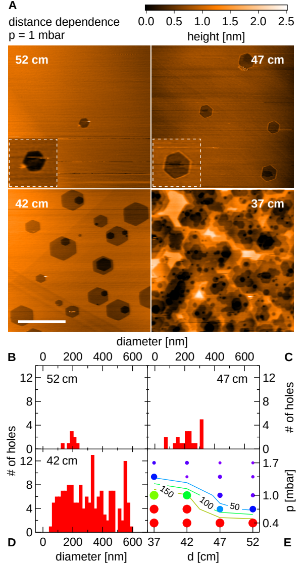
FIG. 1. Distance dependence of graphite exposures (A) AFM images (tapping mode) of graphite surfaces for various distances d , as labeled, all exposed to the plasma for 1 h at p = 1\text{ mbar} and T = 400^\circ\text{C} , all shown on the same color scale. Main panels are 3 \times 3\ \mu\text{m}^2 , scale bar is 1\ \mu\text{m} , insets (dashed white boxes) are 0.25 \times 0.25\ \mu\text{m}^2 . Slight hexagon distortion at 42 cm is an imaging artefact due to drift. (B-D) Histograms obtained from 10 \times 10\ \mu\text{m}^2 scans, showing the number of holes against hole diameter (bin size 20 nm). (E) The size of the circle markers corresponds to the width of the diameter distribution. The color indicates the number of holes, with red corresponding to large number of holes. For samples located within the glowing plasma (red circles), a lower bound of 300 holes and a minimum width of distribution of diameter of 600 nm is shown.
