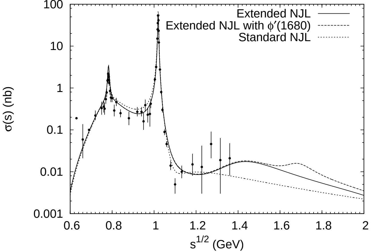
Figure 3: Comparison of the NJL model predictions with the experiment [14] for the e^+e^- \rightarrow \eta\gamma process.
