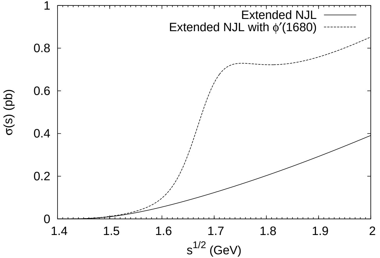
Figure 6: Predictions for the e^+e^- \rightarrow \eta(1405)\gamma process given by the extended NJL model.
