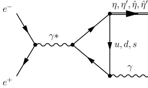
Figure 1: Feynman diagram with photon exchange.
