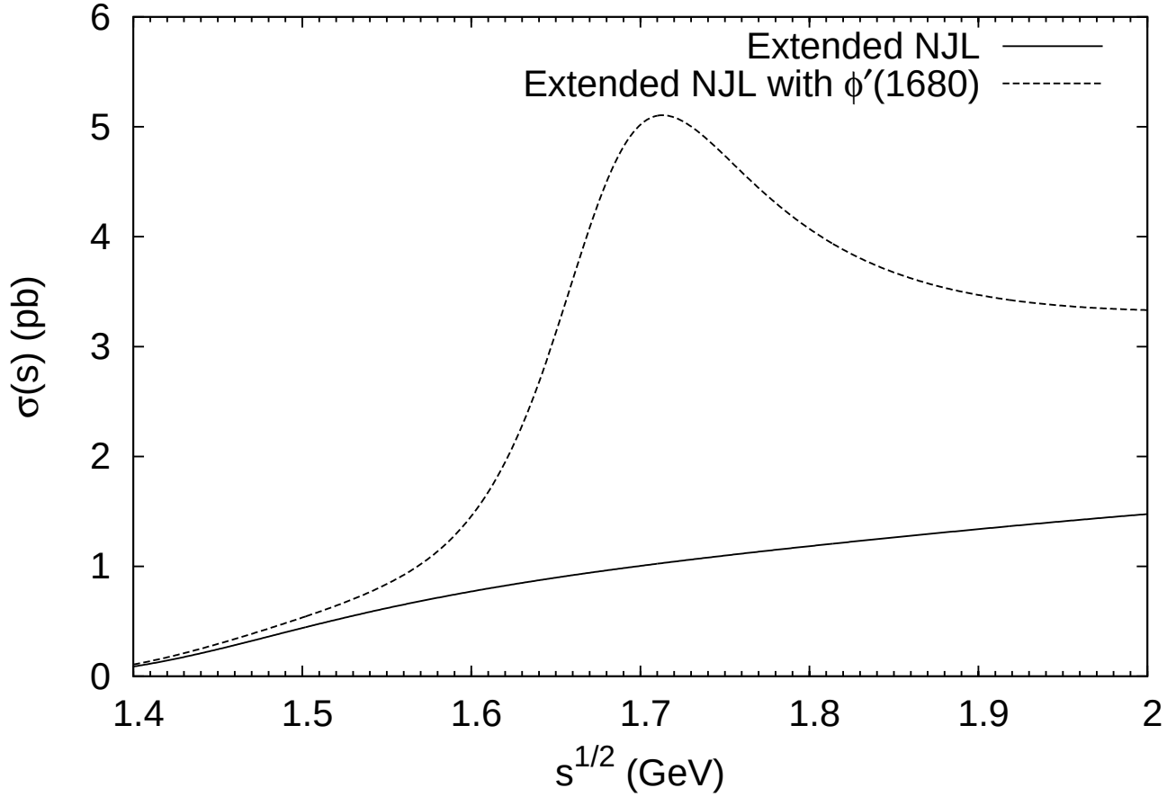
Figure 5: Predictions for the e^+e^- \rightarrow \eta(1295)\gamma process given by the extended NJL model.
