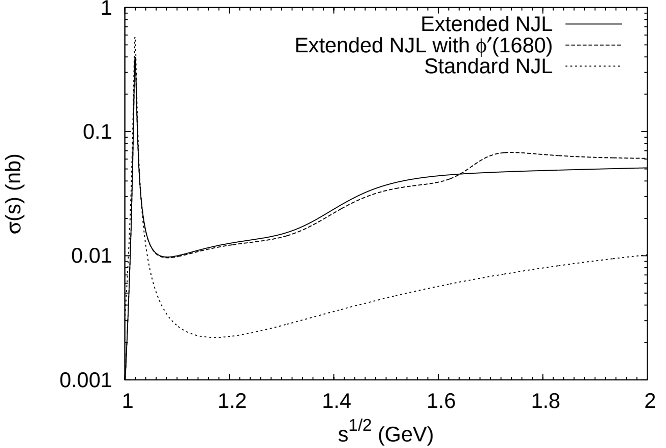
Figure 4: Predictions for the e^+e^- \rightarrow \eta'\gamma process given by the extended and standard NJL models.
