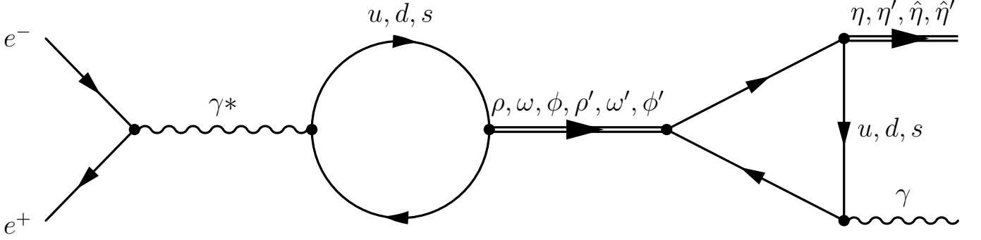
Figure 2: Feynman diagrams with \rho, \omega, \phi, \rho', \omega', \phi' meson exchange.
