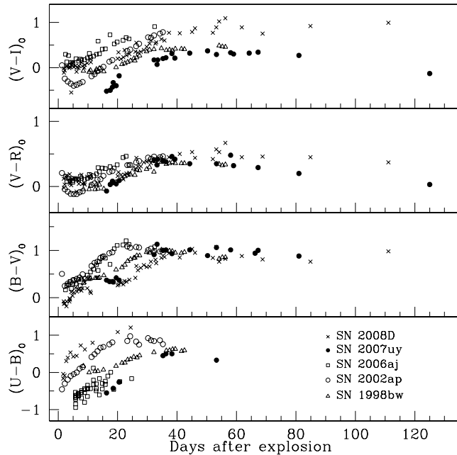
Figure 10. Color evolution of SN 2007uy. Comparison with other Type Ibc events
