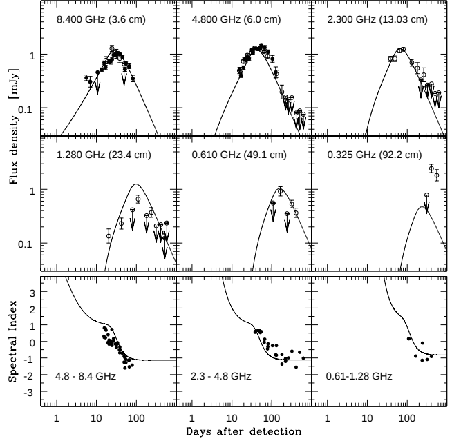
Figure 13. The modeled radio light curve of SN 2007uy. The upper panel shows the variation of radio signal with time. Open circles are the data obtained from van der Horst et al. (2011), whereas the filled circles are VLA data acquired for the present work. The solid curves represent the best fit model. The lower panel shows the variation of spectral index with time.
