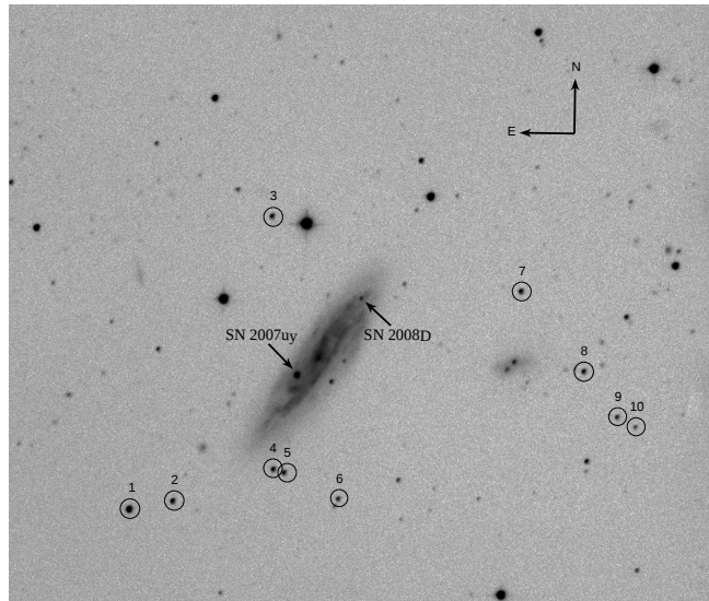
Figure 1. Identification chart of SN 2007uy. The image is about 10 arcmin on a side taken in V-band with the 104-cm Sampurnanand telescope at ARIES, Nainital. The local second-order stars are numbered. North is up and east is to the left.
