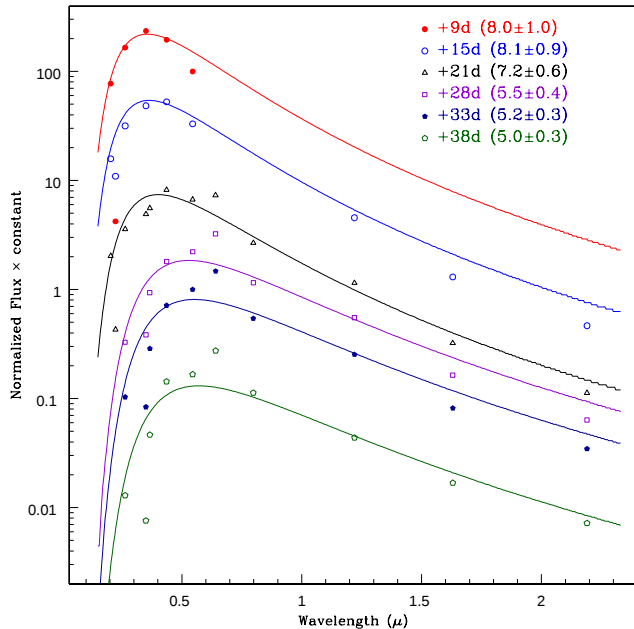
Figure 9. Temporal evolution of observed SED of SN 2007uy. The temperature of each blackbody is mentioned inside the parenthesis, with a temperature-scale 1000K. The one sigma uncertainties are measured by applying the ‘Monte Carlo’ method. The colour version of the figure is available in the online journal.
