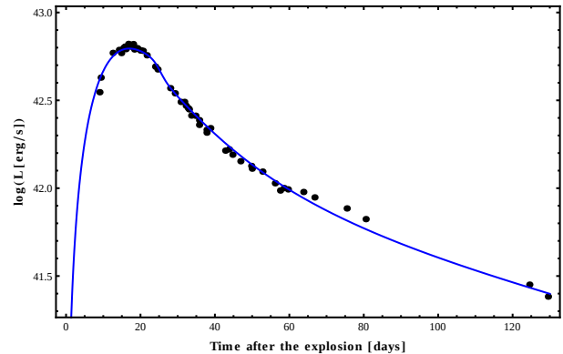
Figure 12. The modeled UVOIR bolometric light curve of SN 2007uy. The black dots are the observed data points. The blue solid line represents the model. The colour version is available in online journal.
