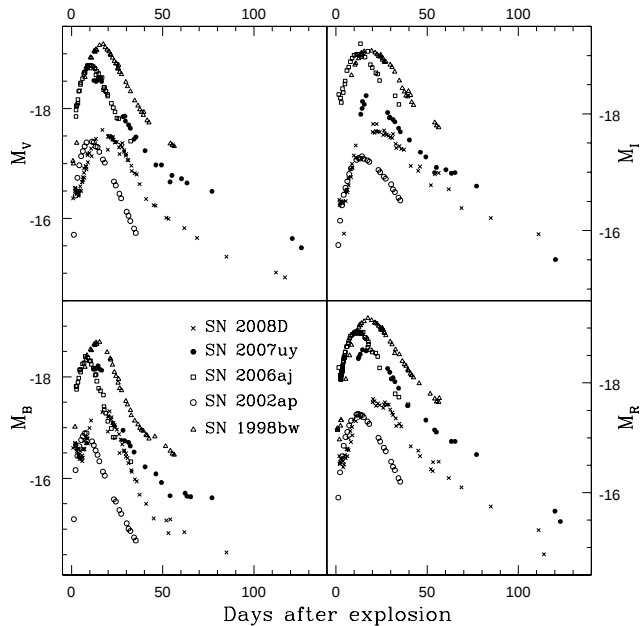
Figure 7. Absolute light curves of SN 2007uy. Comparison with other Type Ib and Ic events.
