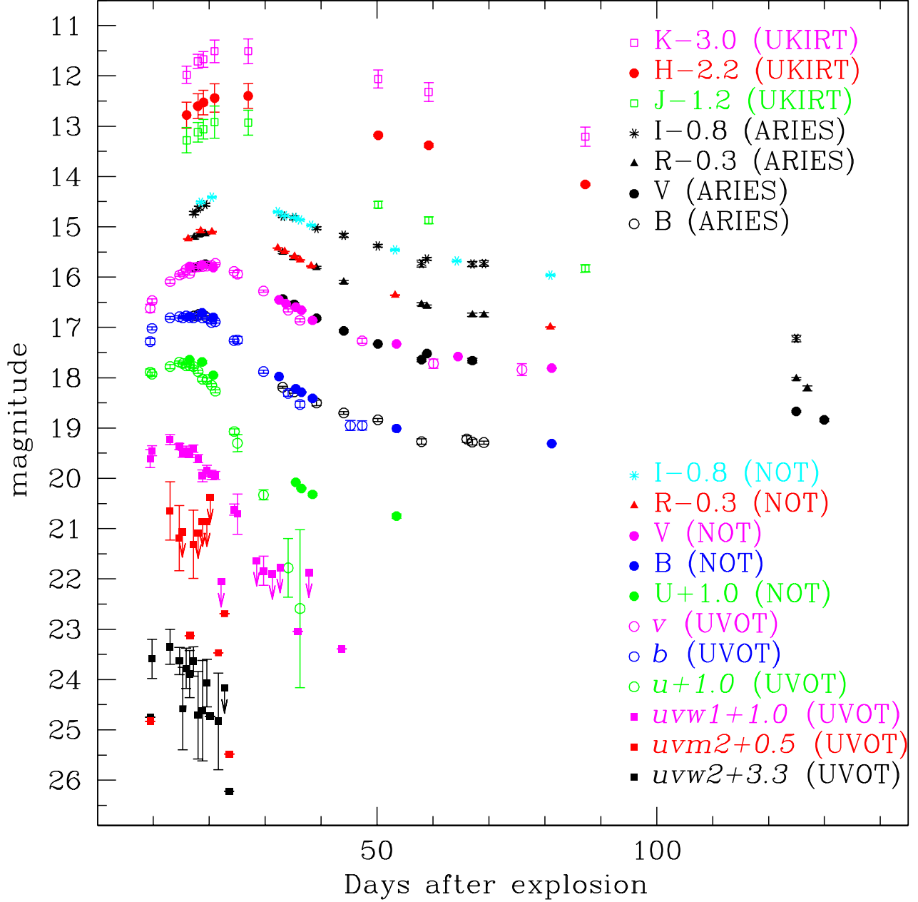
Figure 6. The light curves of SN 2007uy in NIR JHK , Optical UBVRI and uvw2 , uvm2 , uvw1&u , b , v NUV-Optical UVOT bands. The colour version of the figure is available in the online journal.
