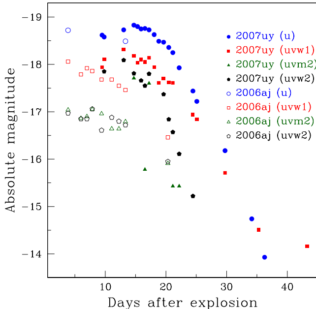
Figure 8. NUV and u band absolute light curves of SN 2007uy. Comparison with Type Ic event SN 2006aj. Data for SN 2006aj were presented by Šimon et al. (2010). The colour version of the figure is available in the online journal.
