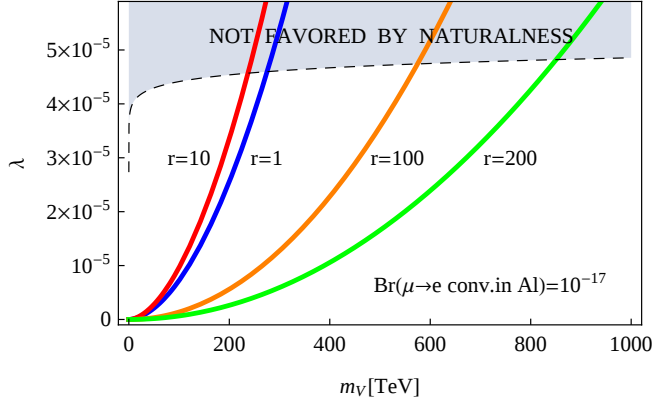
FIG. 6: Same as Fig. 4, but for a branching ratio \text{Br}(\mu \rightarrow e \text{ conversion in Al}) = 10^{-17} .
