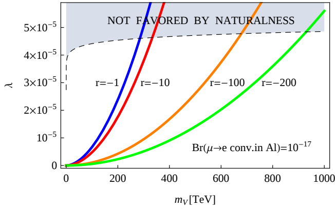
FIG. 7: Same as Fig. 5, but for a branching ratio \text{Br}(\mu \rightarrow e \text{ conversion in Al}) = 10^{-17} .
