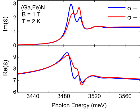
FIG. 2: (color online) The calculated real and imaginary parts of the (Ga,Fe)N ( x = 0.2\% ) dielectric function in B = 1 T and at T = 2 K for both, \sigma^+ and \sigma^- , circular polarizations of the light.
