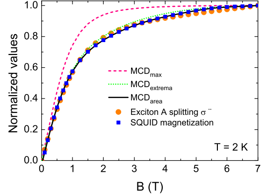
FIG. 5: (color online) Amplitude of the main MCD peak MCD_{\max} (dashed line), the sum of the absolute values of the MCD extrema MCD_{\text{extrema}} (dotted line), integrated area under the MCD curve MCD_{\text{area}} (solid line) plotted together with the exciton A shift in polarization \sigma^- (circles) and magnetization (squares), all normalized by their values at 7 T.
