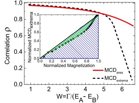
FIG. 7: (color online) Coefficient \rho (Eq. 7) describing the correlation between the magnitudes of magnetization and MCD for \text{MCD}_{\text{area}} (solid line) and \text{MCD}_{\text{extrema}} (dashed line), as defined in Sec. V, plotted vs. the parameter W (Eq. 8) describing the spectral broadening of the excitonic transitions. Good agreement between the magnitude of magnetization and MCD ( \rho > 0.9 ) is maintained up to W \sim 5 and deteriorates for higher W , particularly in the case of \text{MCD}_{\text{extrema}} . Inset: normalized \text{MCD}_{\text{extrema}} vs. normalized magnetization for W = 3.8 . The correlation coefficient \rho is calculated as the ratio of the triangle areas below the dotted and solid lines.
