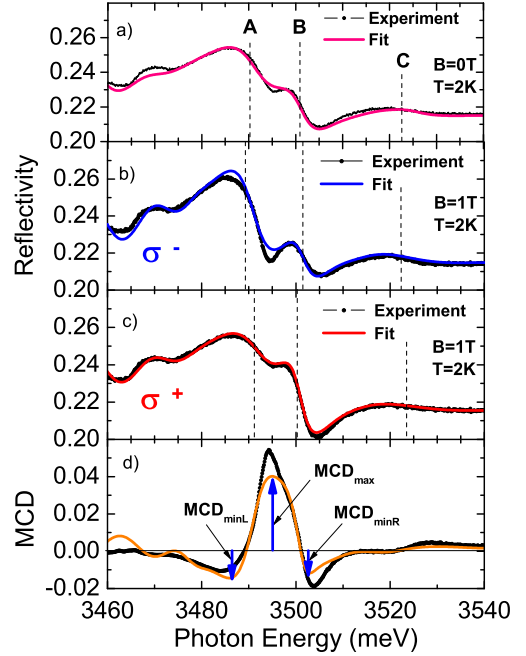
FIG. 3: (color online) Experimental (points) and fitted (solid lines) reflectivity spectra at B = 0 T (a) and at 1 T for \sigma^- (b) and \sigma^+ (c) polarizations. The energies of optical transitions corresponding to the excitons A, B and C are indicated (vertical dashed lines). In panel (d) the experimental (points) and modeled (lines) MCD spectra are given, as determined from the reflectivity spectra shown in panels (b) and (c).
