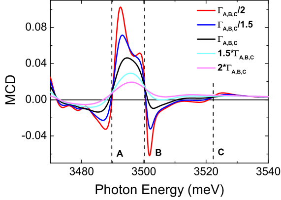
FIG. 6: (color online) Calculated MCD spectra at 1 T for various linewidths of the excitons A , B and C , changed by a factor between 1/2 and 2 . The vertical lines indicate the positions of the excitons in the absence of a magnetic field.
