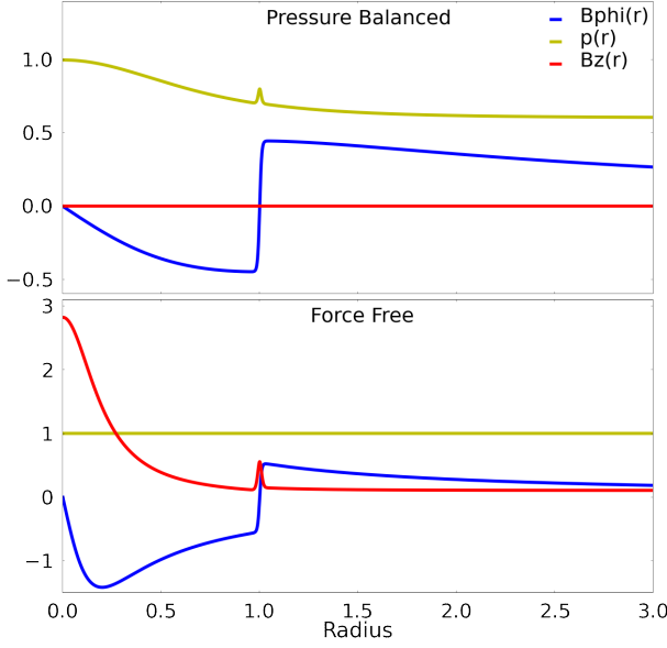
Figure 2. Radial profiles of B_\phi , B_z and p for the pressure balanced (case PB-0) and force-free (case FF-0.2) equilibrium configurations. In both cases the Lundquist number is S = 2.4 \times 10^4 .
