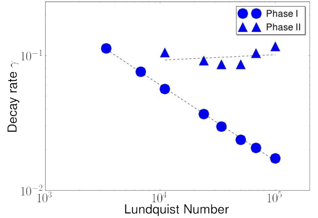
Figure 6. Decay rate \gamma of the magnetic energy as a function of S for case PB-0-2D. For each S values \gamma is computed in phase I (circles) and phase 2 (triangles). The decay rate scales as S^{-1/2} during phase I, and it is nearly independent on S in phase II.
