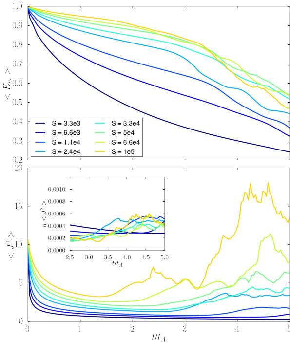
Figure 5. Two-dimensional circular current sheet. (Top panel) Temporal evolution of average magnetic energy E_m normalized to the initial magnetic energy for different values of the Lundquist number. (Bottom panel) Temporal evolution of \langle J^2 \rangle for different values of the Lundquist number. (Inset) Temporal evolution of \eta \langle J^2 \rangle for different Lundquist numbers.
