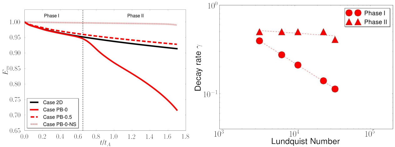
Figure 8. (Left) Temporal evolution of the volume averaged magnetic energy normalized to the initial magnetic energy for case PB-0 (red solid line), case PB-0.5 (dashed line) and case PB-0-NS (dotted line), along with case 2D (black). For all cases the Lundquist number is S = 2.4 \times 10^4 . The black vertical line separates phase I and phase II for case PB-2D. (Right) Decay rate \gamma of the magnetic energy as a function of S for case PB-0. For each S value, \gamma is computed in phase I (circles) and phase 2 (triangles). We note that the decay rate follows the Sweet-Parker scaling during phase I, and is nearly independent on S in phase II.
