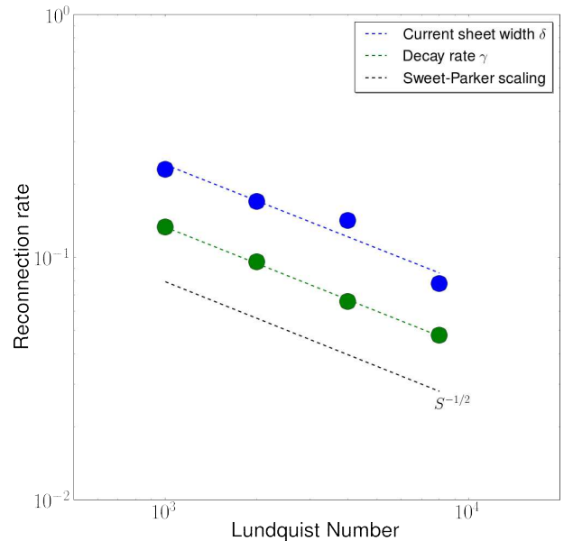
Figure 3. Reconnection rate \eta computed with two different methods: Blue : time average of \delta as a function of S , along with a best fit (dashed line). Green : Magnetic energy decay \gamma as a function of S , along with a best fit (dashed line). The Sweet-Parker scaling \sim S^{-1/2} is plotted in black.
