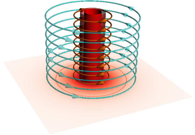
Figure 1. Contour rendering of the density showing the plasma column at t = 0 for the pressure balanced equilibrium. A slice of the density (pseudocolor rendering) on the xy plane ( z = -1 ) is superimposed, showing the maximum of \rho at r_1 (see text). The red and blue circles show magnetic field lines of opposite polarity for B_\phi .
