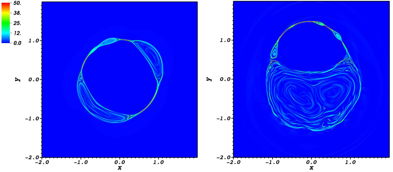
Figure 4. Pseudocolor rendering of the current density J_z for case 2D with S = 1.0 \times 10^5 at t \simeq 2.5t_A (left) and t \simeq 4.8t_A (right). We note the formation of multiple plasmoids and small-sized current sheets due to secondary tearing instability, in a manner similar to the “plasmoid turbulence” described in Loureiro et al. (2012).
