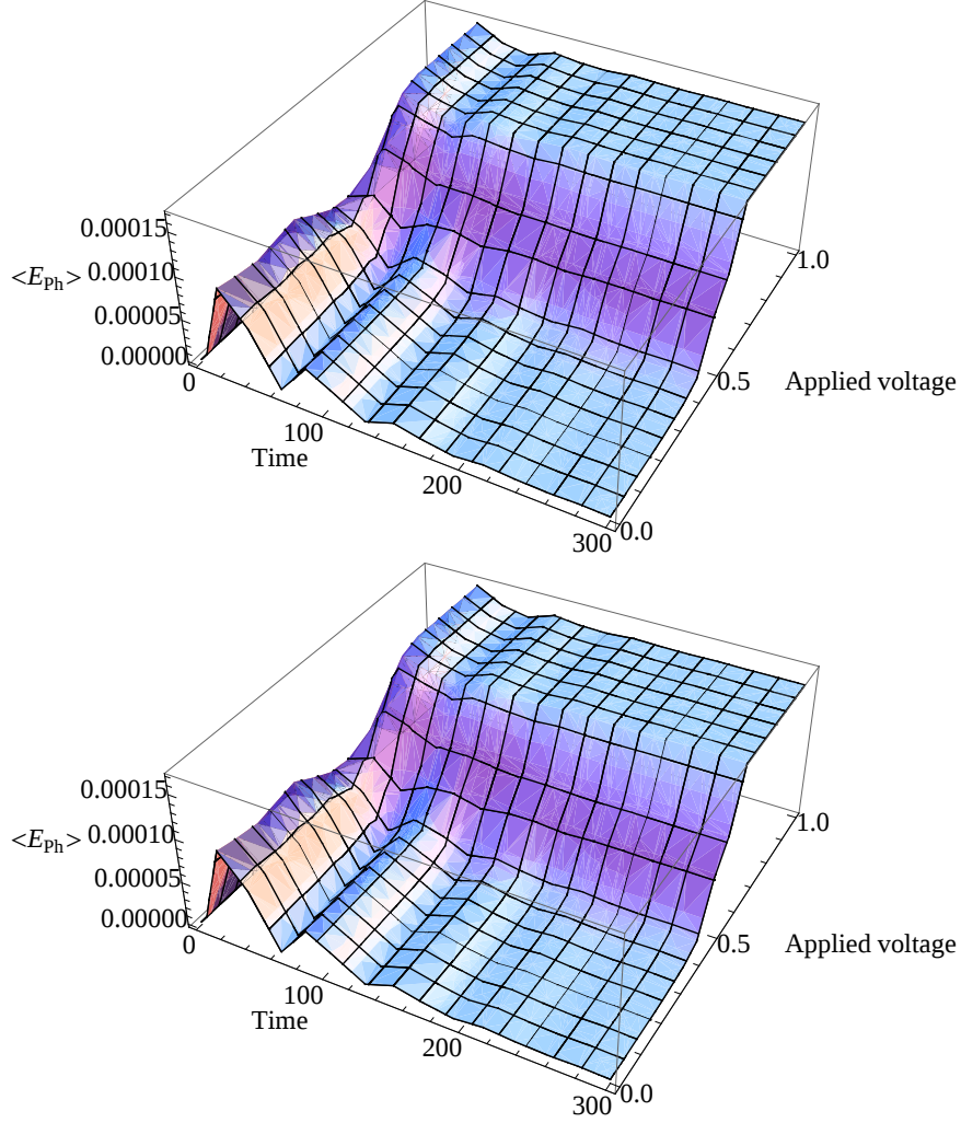
FIG. 6. Average energy transferred to the oscillator as a function of time and left Fermi level for fixed values of \epsilon_0 = 0.5 , \epsilon_{FR} = 0 , \Gamma = 0.01 and for different values of coupling strength: \eta = 0.02 (Fig. 6(a)), and 0.08 (Fig. 6(b)). Units: all the parameters have same dimension as of \hbar\omega .
