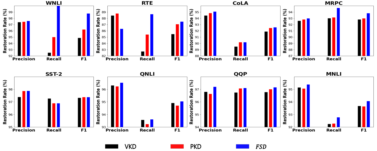
Figure 3: Restoration rate of teachers' predictions in students on the GLUE tasks. MNLI used the matched subset.
