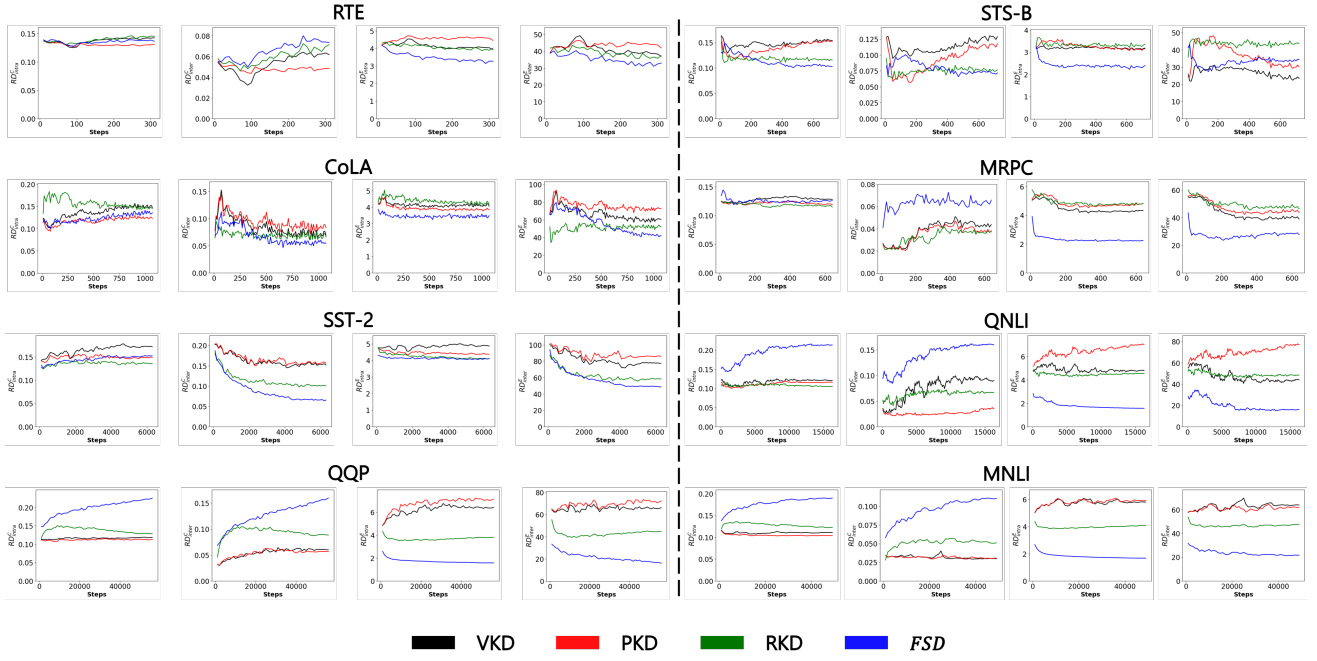
Figure 8: The results of relation difference. Each task shows the results of using different four difference metrics: RD_{intra}^C , second is RD_{intra}^E , third is RD_{inter}^E , and RD_{inter}^E .
