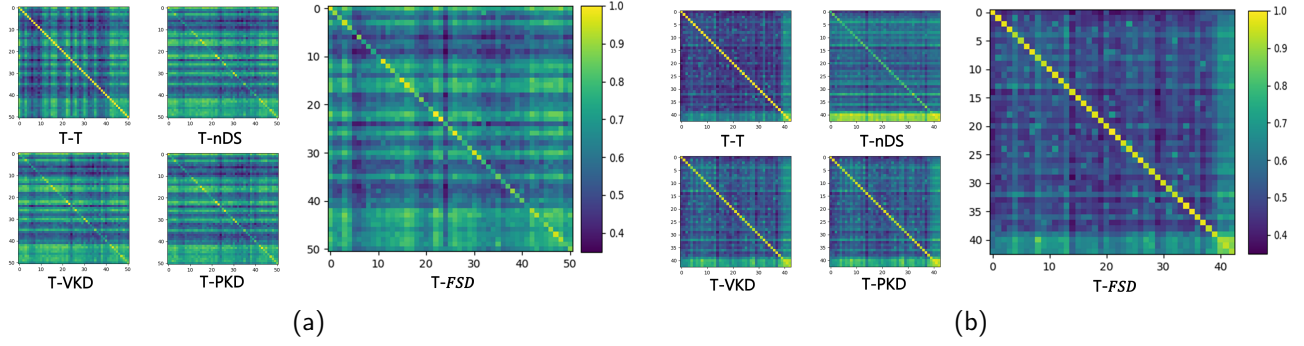
Figure 4: CKA heat maps of GLUE benchmark. CoLA data set result is representative on GLUE benchmark, x-axis, y-axis are indices of mini-batches on the same data set. Each pixel shows the CKA similarity between teacher’s and other model’s representations generated from their mini-batches. In the diagonal lines, the same samples are used for the generation. Right side bar shows the normalized range of CKA similarities observed in each task. (a) is a CoLA case and (b) is a SST-2 case. The heat maps of all the other tasks are in Appendix.
