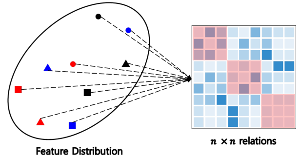
Figure 2: The difference of covered relations between a local structure and a global structure is shown. The blue blocks of the right-side matrix are relations of the global structure in the full batch. The red blocks are found in mini-batches (local structure). Various colored and shaped markers indicate features and the matrix shows relations over the features.
