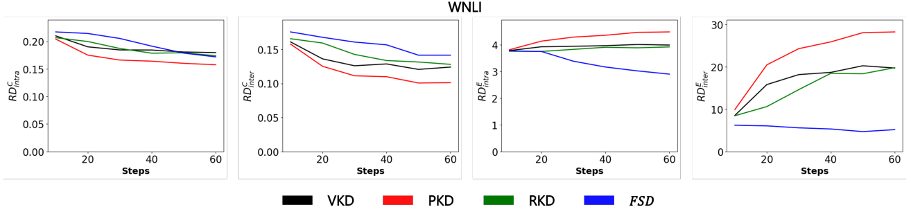
Figure 6: The results of relation difference. Each task shows the results of using different four difference metrics: RD_{intra}^C , second is RD_{inter}^C , third is RD_{intra}^E , and RD_{inter}^E . First row, WNLi, results are representative. The results of all the other tasks are in Appendix.
