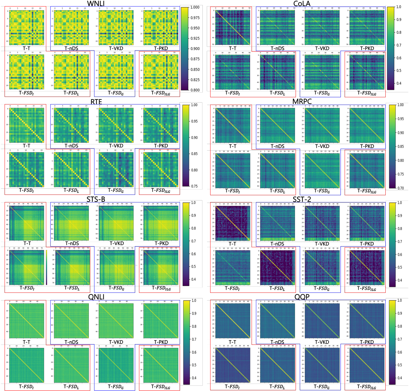
Figure 7: CKA heatmap of GLUE benchmark. Red box represents teacher closed methods and blue represents no-Distillation-Student closed methods.
