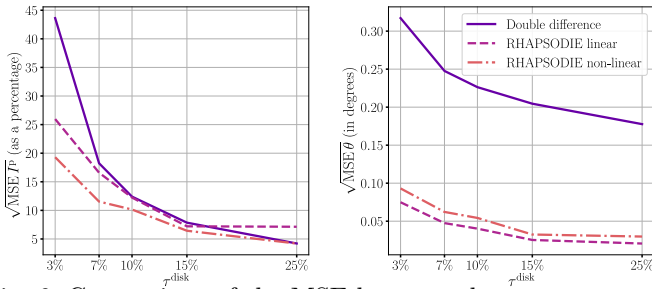
Fig. 6: Comparison of the MSE between the true map and the estimated map of the polarized intensity I^P and of the angle of polarization \theta for the Double Difference and the linear and non-linear RHAPSODIE methods without deconvolution.
