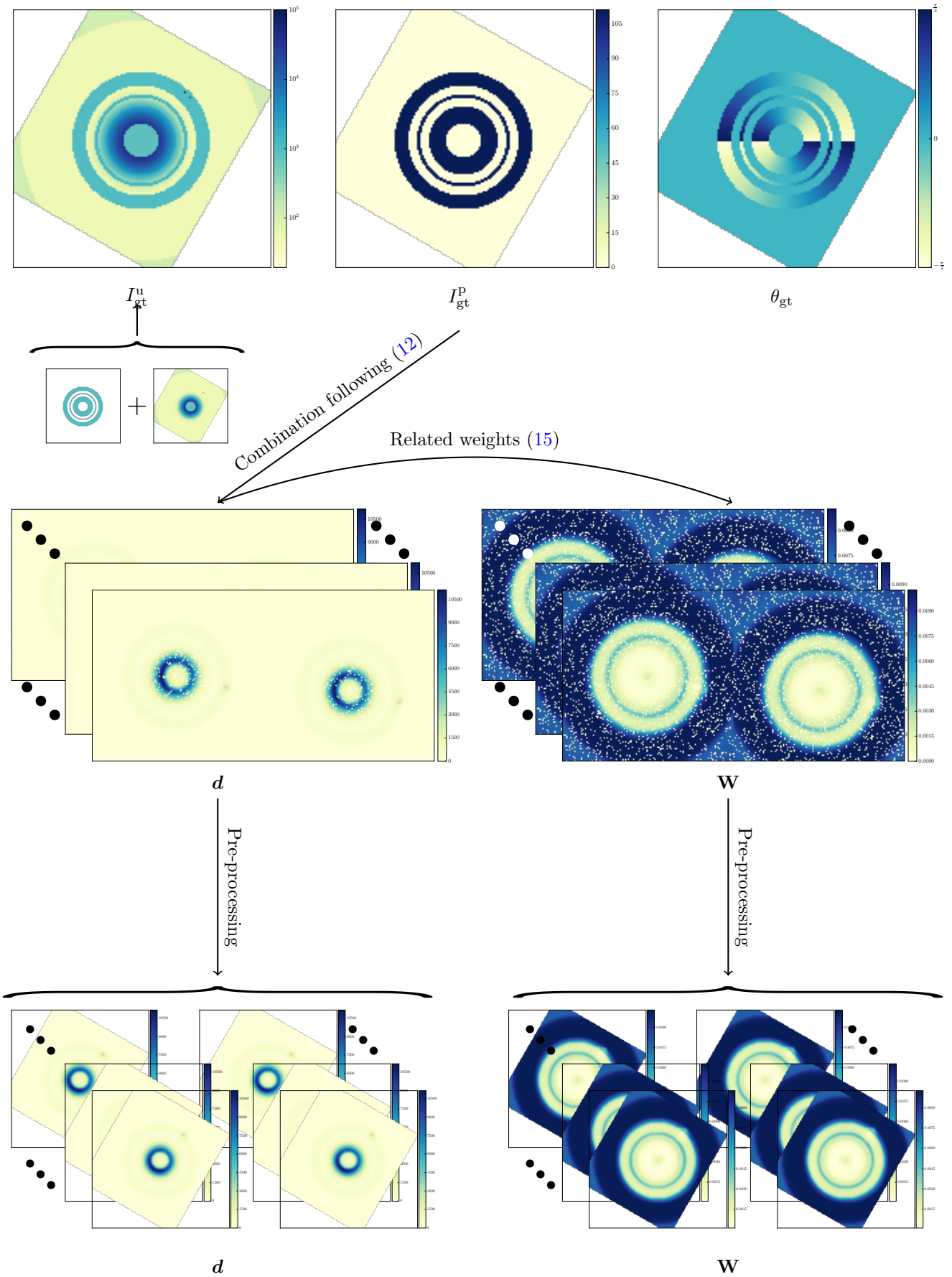
Fig. A.2: Schematic describing the process of the data simulation. Starting from synthetic maps I_{\text{gt}}^u , I_{\text{gt}}^p , and \theta_{\text{gt}} based on a disc model, we generate artificial calibrated and pre-processed datasets d and associated weights W , illustrated here for \tau^{\text{disk}} = 10\% .
