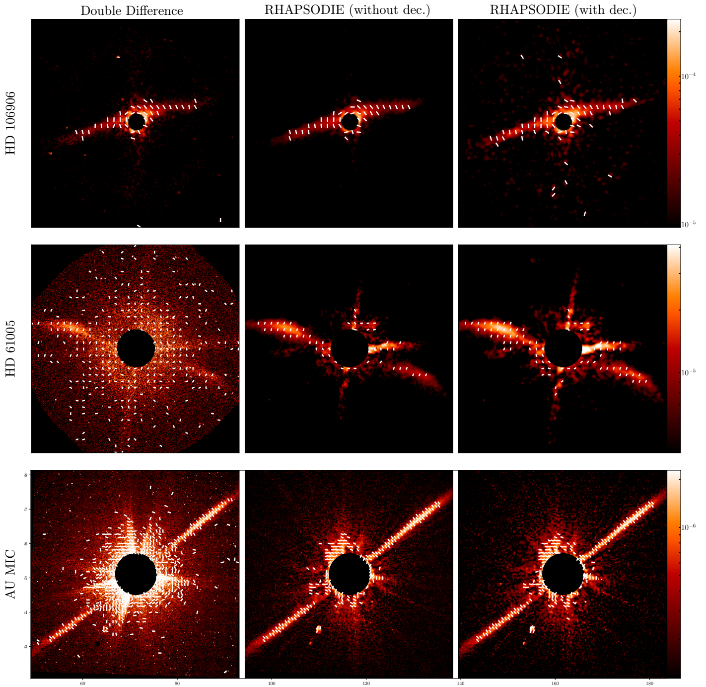
Fig. 16: Reconstructions of the polarized intensity I^P of the debris disks HD 106906, HD 61005, and AU MIC. From the left to the right, the reconstructions have been obtained with the Double Difference, RHAPSODIE without deconvolution and RHAPSODIE with deconvolution . The maps are displayed in logarithmic scale and normalized in contrast to the unpolarized stellar flux. The pixels lying underneath the coronagraph are masked in black. North is up and East is to the left in all frames.
