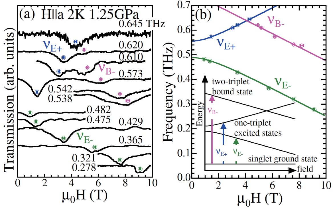
Fig. 1. (Color online) Typical frequency dependence of ESR spectra (a) and frequency-field diagram (b) obtained at 1.25 GPa and 2 K for H||a. Inset: schematic of the energy-field diagram and the observed ESR transitions.
