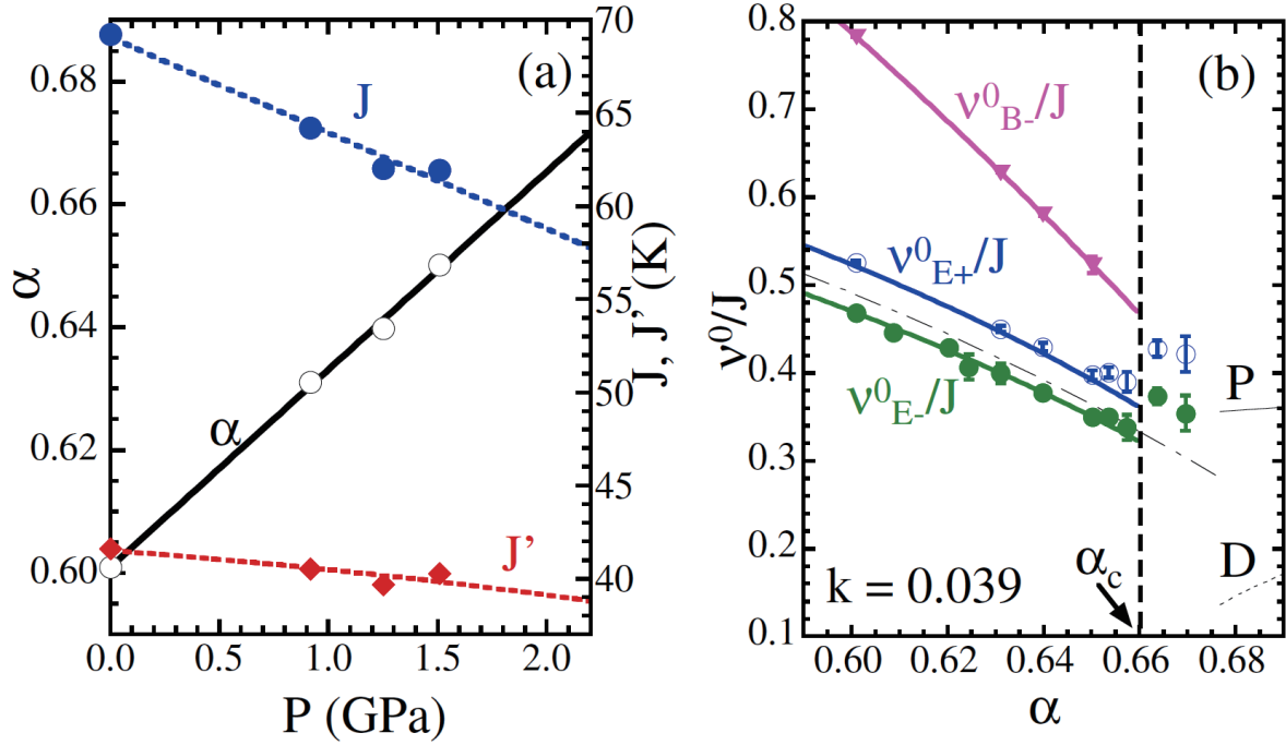
Fig. 3. (Color online) (a) Pressure dependence of J , J' and \alpha . (b) Gap energies v^0_{E\pm} and v^0_{B-} normalized by J as a function of \alpha . The symbols correspond to those in Fig. 2(b). Thick lines are obtained by the exact diagonal calculation with k = 0.039 . Thin lines are the results obtained in Takushima et al. 12) See text for details.
