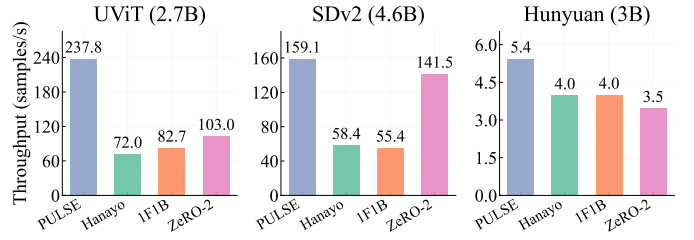
(b) Throughput on a 8-node Ascend cluster
