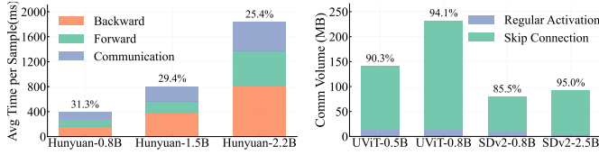
Fig. 2: Time breakdown of ZeRO3 for training Hunyuan-DiT models on 8 V100 GPUs.
