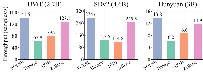
(a) Throughput on a 2-node V100 Cluster
