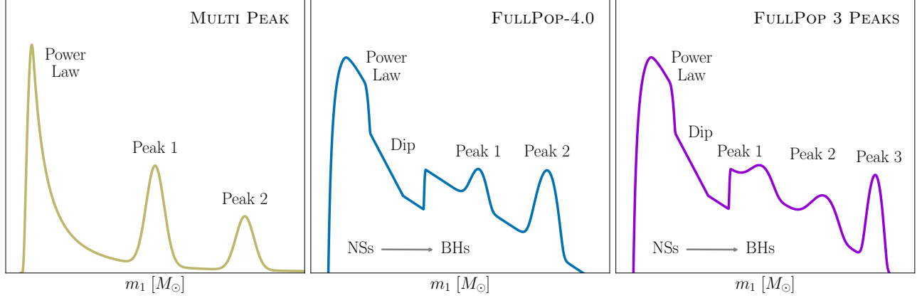
Figure 1. Qualitative graphical representation of the three source-frame mass models considered in this paper and described in Section 2.3 and Appendix A. The mass distribution model displayed in the first panel represent the mass ranges of BHs, while the second two panels include both BHs and NSs. The mass ranges shown are not to scale.
