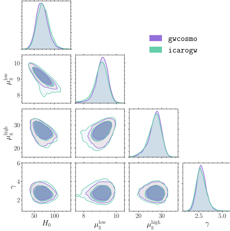
Figure 11. Spectral siren reduced corner plot of the Hubble constant and a subset of the FULLPOP-4.0 model mass parameters obtained with gwcosmo and icarogw. The contours indicate the 68.3% and 90% CR.
