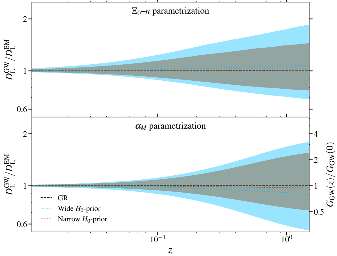
Figure 7. Reconstructed ratio D_L^{\text{GW}}/D_L^{\text{EM}} as a function of cosmological redshift z , for the two modified gravity parametrizations considered, \Xi_0-n and \alpha_M . The blue (brown) bands indicate wide and narrow H_0 -prior results, respectively (see Table 4 for details). In all cases the contours show the 90% CI with median (dotted curve) reconstructed distance ratio from spectral siren analyses with the FULLPOP-4.0 mass model. The black dashed curve represents the GR limit. Note that the reconstructed distance ratio is asymmetric at higher redshifts. The additional righthand y -axis on the lower panel converts the constraints on the \alpha_M parametrization into an effective gravitational coupling, which is discussed in section 2.4.2 and Appendix F. This interpretation is not applicable to the \Xi_0-n parametrization.
