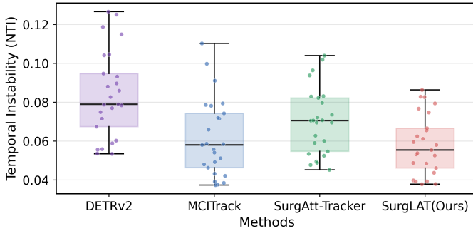
Fig. 5. Comparison of motion-aware temporal instability across 25 validation videos. Lower values indicate smoother and more GT-consistent attention prediction.
