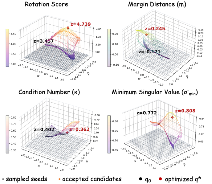
Fig. 6. Visualization of the null-space search for initial configuration optimization. q^* achieves improved rotational capability and a larger joint-limit margin while preserving comparable local conditioning properties.
