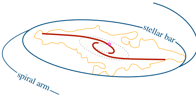
Figure 5. Sketch of the central structures in the host galaxy of SLSN PTF10tpz. The blue ellipse shows the stellar bar of the galaxy. The orange contour shows the extent of the molecular gas in the bar, as presented in the right panel of Figure 2. The two dotted gray ellipses represent the two ellipses in Figure 3. The two red spirals show the gas lanes along which the molecular gas flows toward the galaxy center. The position of the SLSN is marked by a magenta circle.
