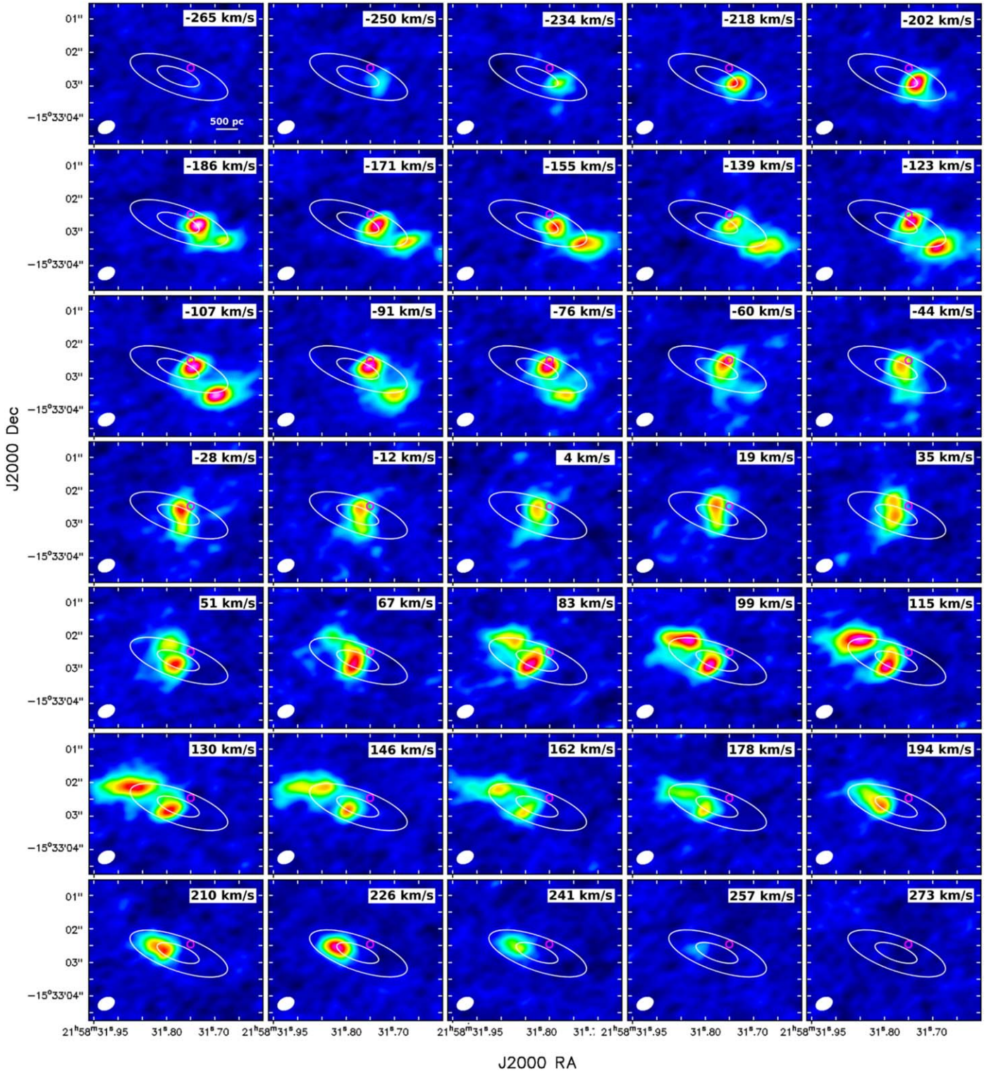
Figure 3. CO emission flux in successive 16 \text{ km s}^{-1} velocity channels. Each map covers the area marked with the dashed blue box in the right panel of Figure 2. The two white ellipses are there to help follow the path of the emission through the velocity channels, within the central few kiloparsecs of the galaxy. The orientations and axial ratios of the two ellipses are same as those of the outermost isophotes of the optical disk of the galaxy. The position of the SLSN is marked with a magenta circle with a radius indicating the uncertainties on the SLSN coordinates. The beam is shown in the bottom left corner of each panel.
