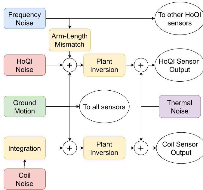
Figure 5. A block diagram illustrating different noise sources present in the device. Uncorrelated noises that cannot be suppressed using a huddle test are shown in red, correlated motion is shown in green. The frequency noise is common between all HoQI-L4C sensors, while thermal noise is common between the interferometric readouts and coil readouts on an individual sensor but are uncorrelated between multiple sensors.
