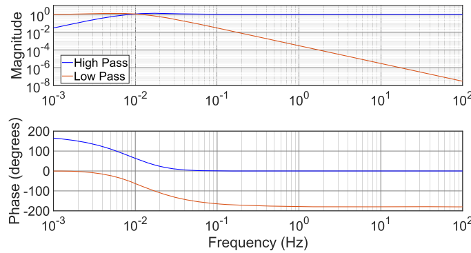
Figure 8. Figure showing the new high and low pass filters generated by optimising equation (4).
