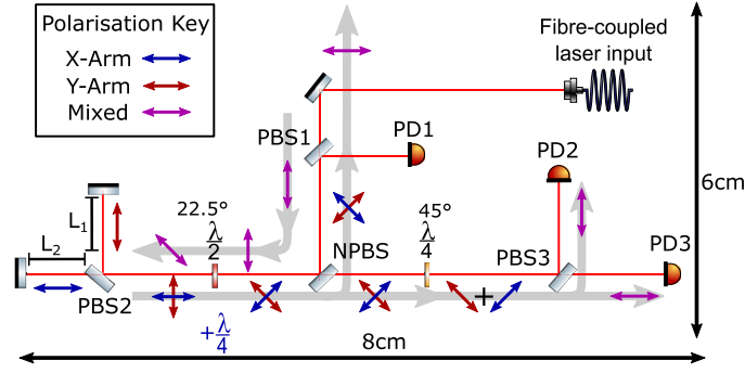
Figure 1. The layout of HoQI used as an interferometric readout on the modified L-4C.
