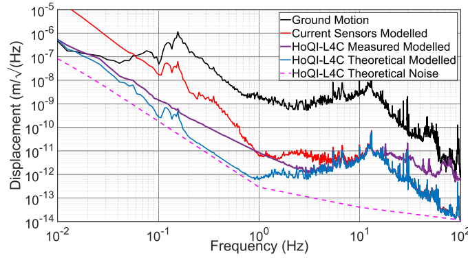
Figure 9. A comparison between the isolation performance using current sensors (red) with the measured and theoretical noise of HoQI-L4Cs (purple and blue respectively). The noise used in the purple and blue traces also include the theoretical suspension thermal noise of the device. The theoretical inertial sensor noise and input ground motion are shown in dashed-magenta and black respectively.
