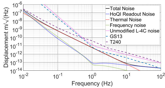
Figure 3. A noise budget of the optical inertial sensor. The interferometer readout noise (blue), structural thermal noise (red) and frequency noise (green) are summed in quadrature to produce the expected resolution of the optical L-4C (black). For comparison the resolution of an L-4C with coil readout is shown in magenta, the GS13 shown in dashed blue and the T240 in dashed purple.
