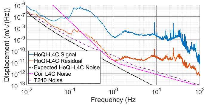
Figure 7. The amplitude spectral density of a HoQI-L4C when exposed to ground motion (blue). Here the measured and predicted resolution of the HoQI-L4C (red, black) with other commercial sensors. The residual signal is generated by subtracting common motion between multiple sensors from a single HoQI-L4C.
