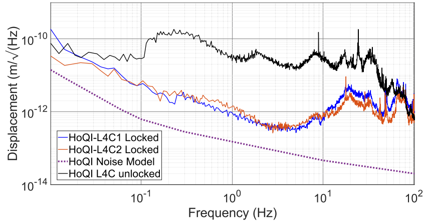
Figure 6. The amplitude spectral density of the displacement measured by HoQI with L-4C mass locked (blue, red). The unlocked interferometer signal with the device exposed to ground motion is shown in black for comparison. In all traces the coherent information has been removed using multiple sensors. The mechanical response of the sensor has not been accounted for and the thermal noise is not included. The expected interferometer noise is shown in dashed purple.
