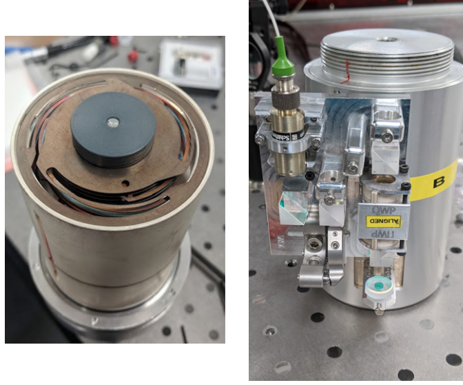
Figure 2. (a) Image showing the internal leaf springs of the L-4C during modification. (b) Prototype version of HoQI used as a readout for an inertial sensor. The baseplate measures 8 \times 6 cm and is fixed to the side of an L-4C geophone.
