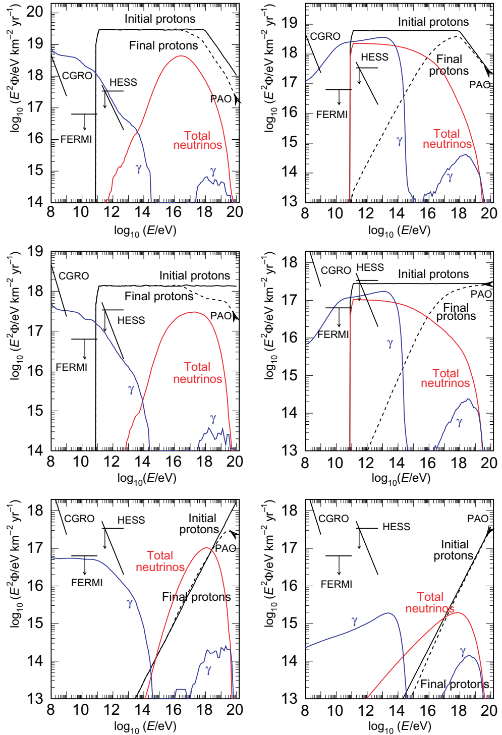
Figure 1. Particle fluxes F(E) from Cen A normalized to the PAO data as a function of the energy E . Top panels: broken power-law with \alpha = 2 and 2.7 and break energy E_b = 10^{18} \text{ eV} ; middle panels: \alpha = 2 ; bottom panels: \alpha = 1.2 ; left panels: acceleration close to the core; right panels: in the jet; the initial protons (solid black line), final protons (dashed black line), photons (blue line), and sum of all neutrinos (red line).
