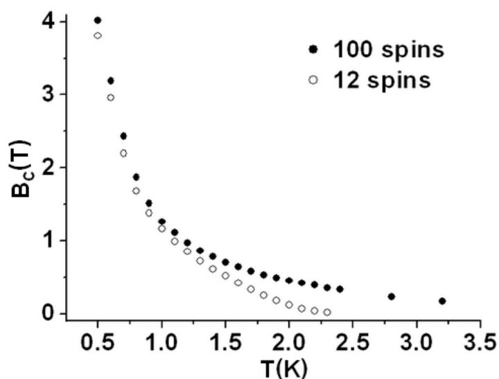
Figure 8. Temperature dependence of coercive field B_c for 2D hexagonal-ordered arrays of N = 12 and 100 spins. The parameters of the Hamiltonian (1) are: K = 1.0 meV, J = -0.3 meV and \mu = 3.2\mu_B .
