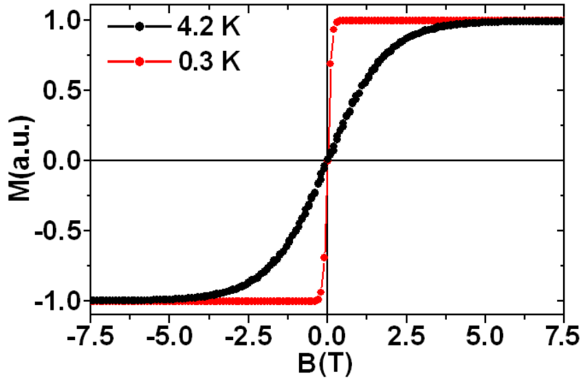
Figure 10. Magnetization response for a single Co adatom on Pt(111) at 0.3 and 4.2 K. The following parameters are used for simulations: \nu_1 = 10^4 Hz, K = 9.3 meV, \mu = 3.8\mu_B , B_0 = 7.5 T and dB/dt = 0.01 T s ^{-1} .
