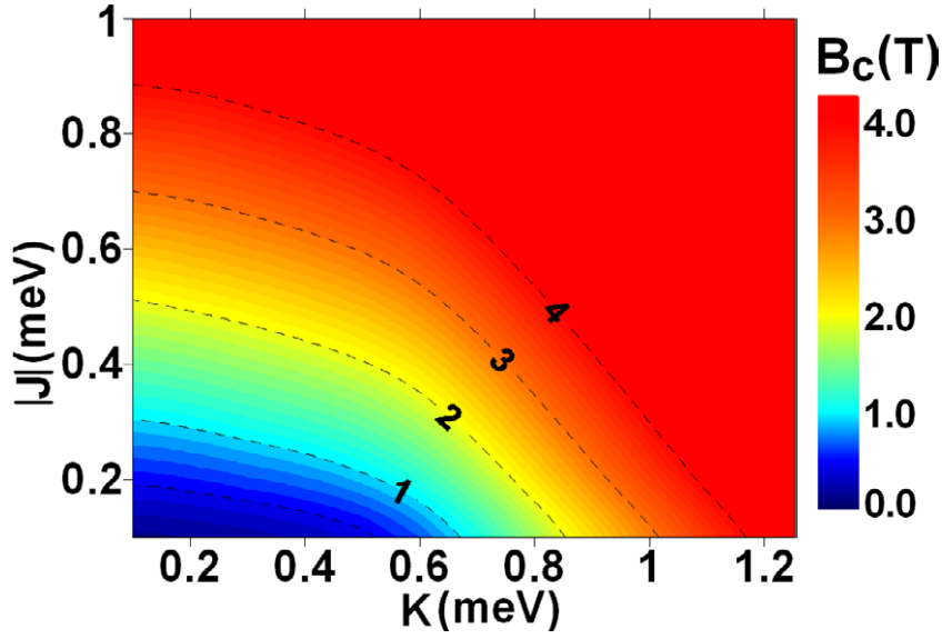
Figure 9. Dependence of coercive field B_c for a 2D hexagonal-ordered array of N = 100 spins on the MAE K and exchange coupling constant J . The diagram is obtained for T = 0.5 K. Dashed curves represent the equipotential lines of coercive field B_c of the corresponding magnitude (see thermometer).
