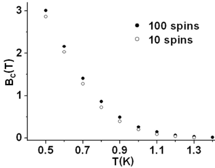
Figure 5. Temperature dependence of coercive field B_c for the 1D chains of N = 10 and 100 spins. The parameters of the Hamiltonian (1) are: K = 1.0 meV, J = -0.3 meV and \mu = 3.2\mu_B .
