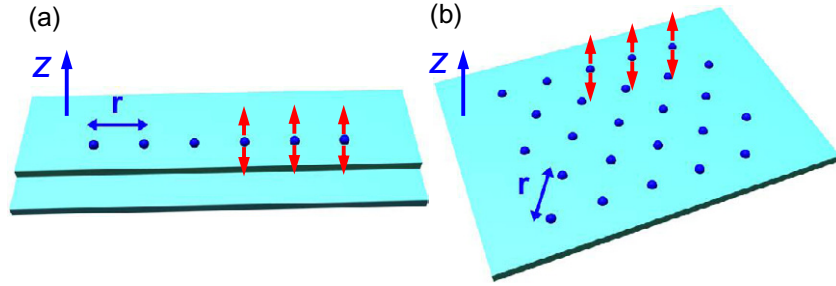
Figure 3. A schematic view of two systems considered within our study: (a) finite 1D chain of equidistantly separated spins and (b) 2D hexagonal-ordered array of equidistantly separated spins. We suppose that both systems represent atomic structures stabilized by the substrate-mediated LRI (figure 2). The easy magnetization axis of an individual adatom is considered to be collinear to the vector Z . Spin orientations along and opposite to the easy axis are demonstrated using red arrows.
