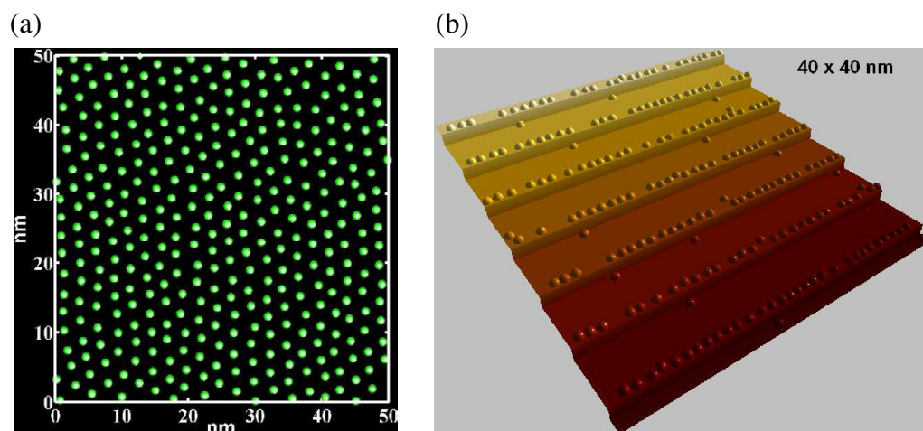
Figure 2. Nanostructures of individual adatoms stabilized by the substrate-mediated LRI. (a) Superlattice of Ce adatoms on Ag(111) [52, 53, 58], (b) monatomic Fe wires in the vicinity of descending Cu(111) steps [60]. The interatomic separation in these nanostructures corresponds to the position of the first local minimum B in the ‘adatom–adatom’ LRI potential (figure 1).
