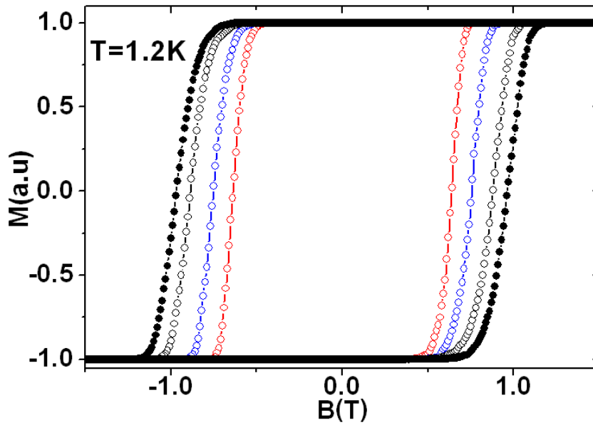
Figure 12. Effect of QT on the magnetization response for the 2D hexagonal-ordered array of N = 100 spins at T = 1.2 K. Black circles correspond to v_1 = 0 (absence of QT), white circles to v_1 = 10^5 Hz, blue circles to v_1 = 10^6 Hz and red circles to v_1 = 10^7 Hz. The values of the parameters of the Hamiltonian (1): K = 1.0 meV, J = -0.3 meV and \mu = 3.2\mu_B .
