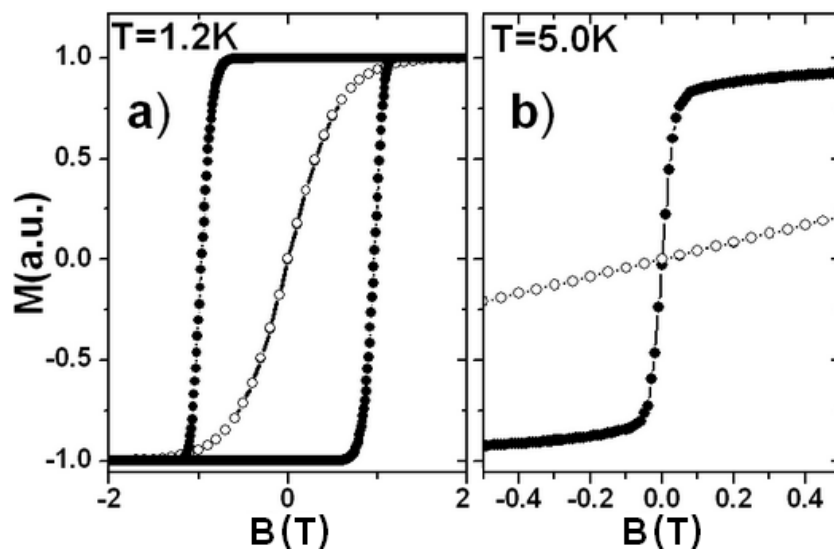
Figure 7. Magnetization response to the external magnetic field for the 2D hexagonal-ordered array of N = 100 spins at two temperatures: (a) 1.2 K, (b) 5.0 K. Black circles correspond to the following parameters of the Hamiltonian (1): K = 1.0 meV, J = -0.3 meV and \mu = 3.2\mu_B , while white circles correspond to: K = 1.0 meV, J = 0 meV and \mu = 3.2\mu_B .
