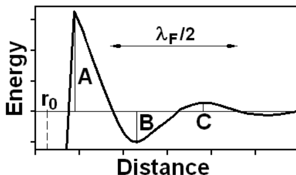
Figure 1. Schematic description of the LRI energy between two adatoms on a (111) noble metal surface supporting 2D free electron gas. Repulsive barriers A and C and attractive minimum B are marked. Distance r_0 corresponds to the NN separation between the adatoms.
