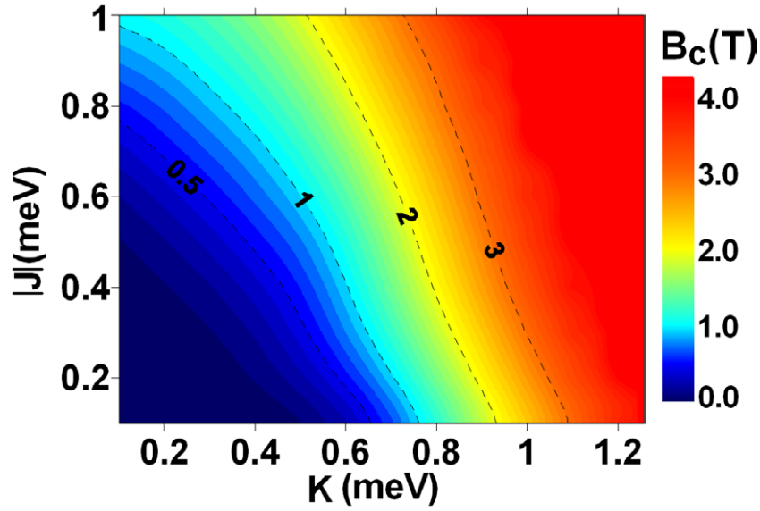
Figure 6. Dependence of coercive field B_c for the chain of N = 100 spins on the MAE K and the exchange coupling constant |J| ( J < 0 ). The diagram is obtained for T = 0.5 K. Dashed curves represent the equipotential lines of coercive field B_c of the corresponding magnitude (see thermometer).
