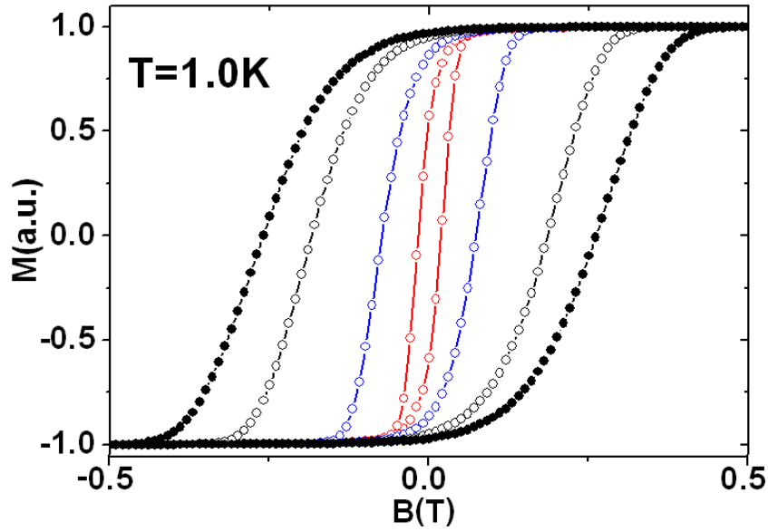
Figure 11. Effect of QT on the magnetization response for the 1D chain of N = 100 spins at T = 1.0 K. Black circles correspond to v_1 = 0 (absence of QT), white circles to v_1 = 10^4 Hz, blue circles to v_1 = 10^5 Hz and red circles to v_1 = 10^6 Hz. The values of the parameters of the Hamiltonian (1): K = 1.0 meV, J = -0.3 meV and \mu = 3.2\mu_B .
