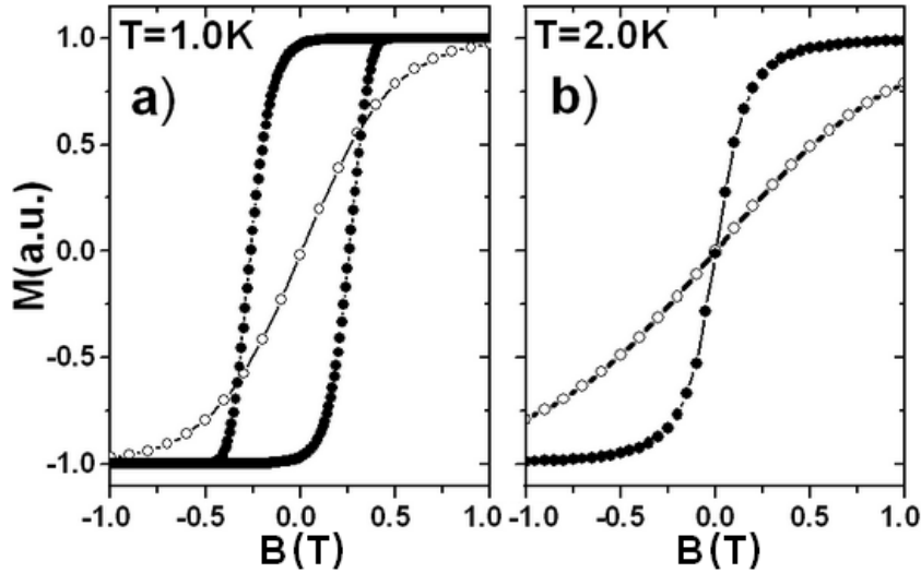
Figure 4. Magnetization response to the external magnetic field for the 1D chain of N = 100 spins at two temperatures: (a) 1.0 K and (b) 2.0 K. Black circles correspond to the following values of parameters of the Hamiltonian (1): K = 1.0 meV, J = -0.3 meV and \mu = 3.2\mu_B , while white circles correspond to: K = 1.0 meV, J = 0 meV and \mu = 3.2\mu_B .
