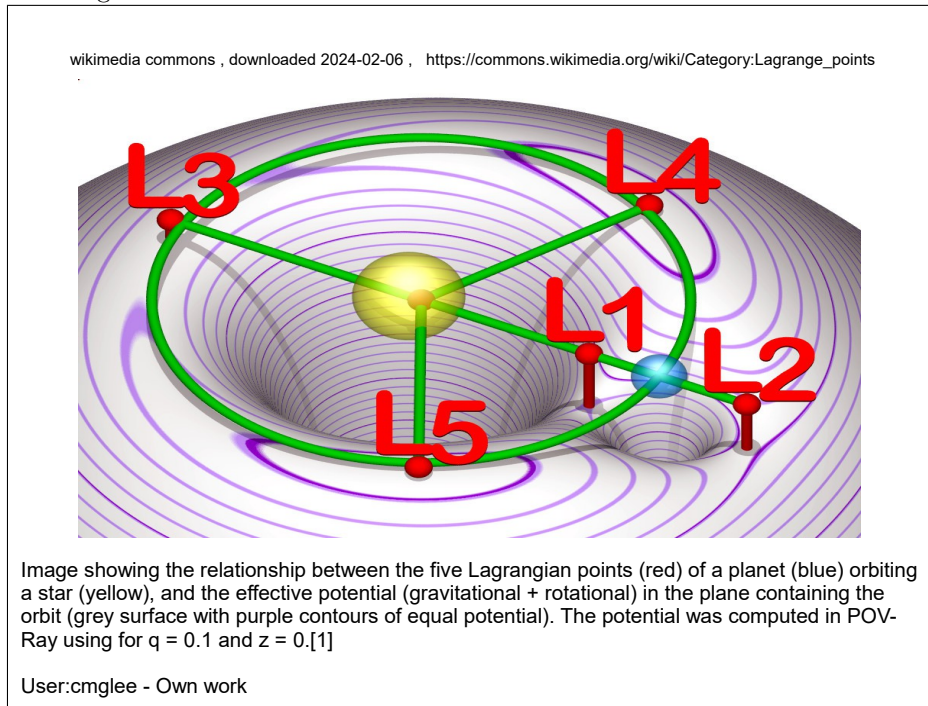
Figure 5: Lagrange points showcase from [46], wikimedia commons, thanks to user cmglee
